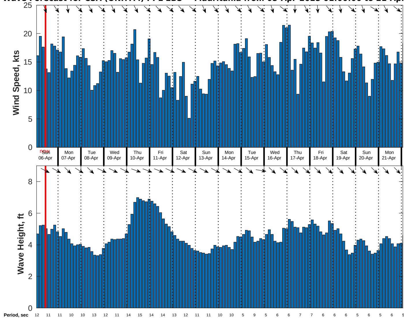
Wind & Wave Forecast for CSA (ONHYM) PPL EBS - Mauritania from 05-Apr-2025 01:00:00 to 21-Apr-2025 01:00:00
