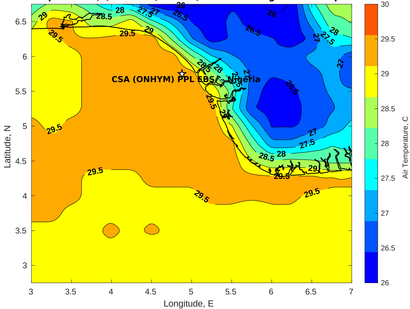
Air Temperature (C) for CSA (ONHYM) PPL EBS - Nigeria at 05-Apr-2025
