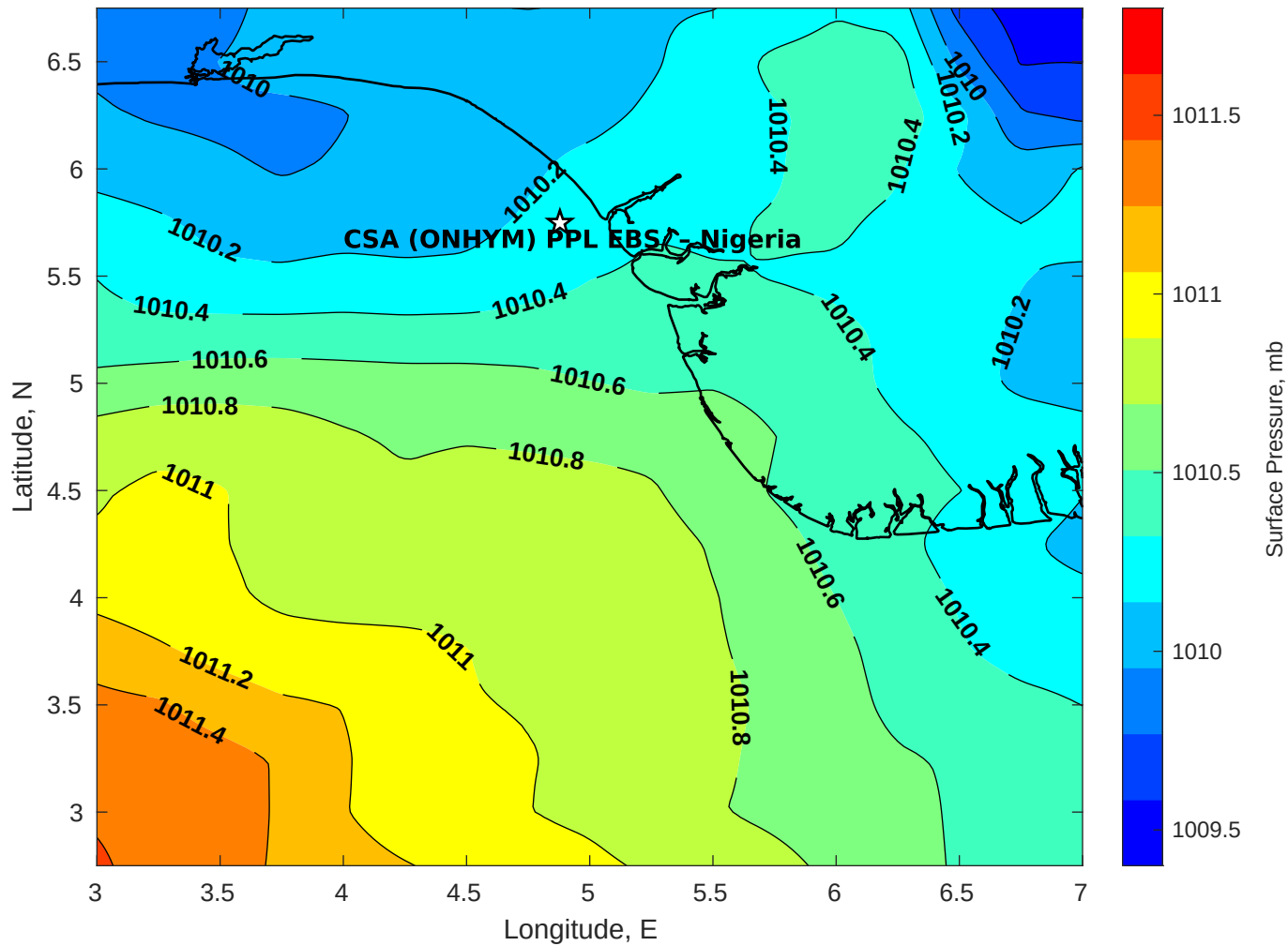
Surface Pressure (mb) for CSA (ONHYM) PPL EBS - Nigeria at 05-Apr-2025 00:00:00
