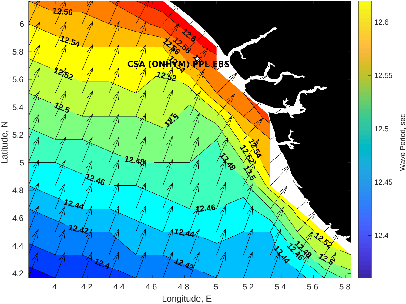
Wave Period (sec) for CSA (ONHYM) PPL EBS - Nigeria at 05-Apr-2025 09:00:00
