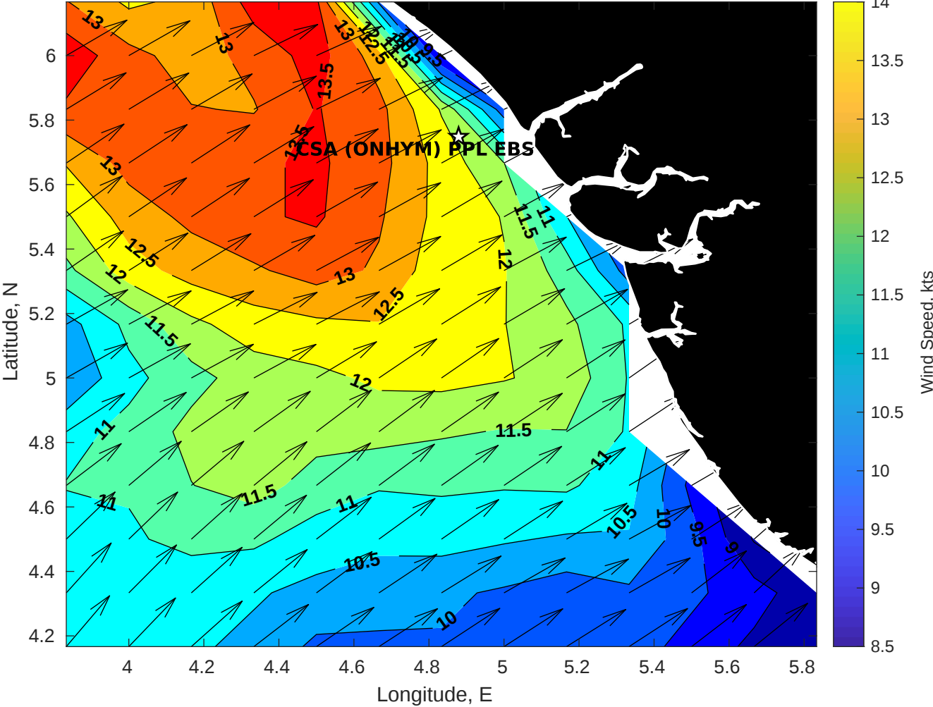
Winds (kts) for CSA (ONHYM) PPL EBS - Nigeria at 05-Apr-2025 09:00:00
