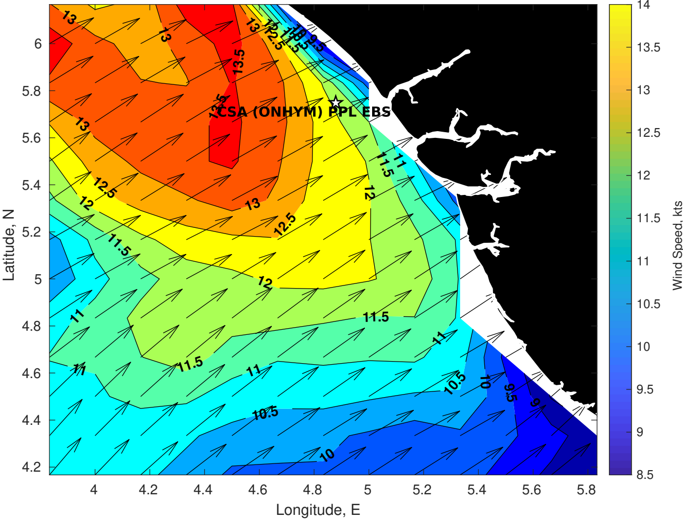
Winds (kts) for CSA (ONHYM) PPL EBS - Nigeria at 05-Apr-2025 09:00:00
