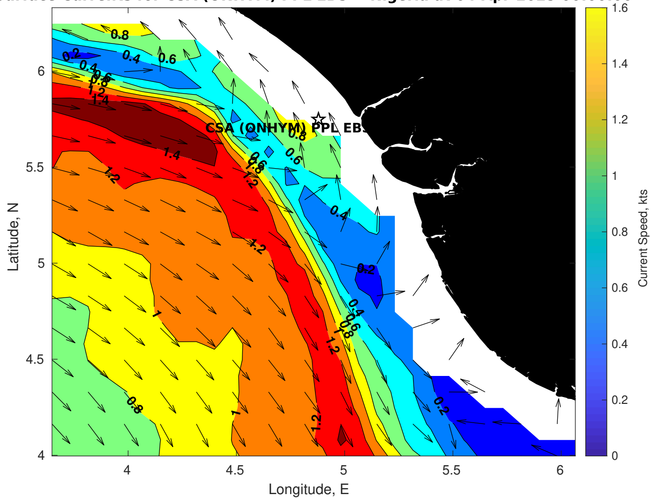
Surface Currents for CSA (ONHYM) PPL EBS - Nigeria at 04-Apr-2025 00:00:00
