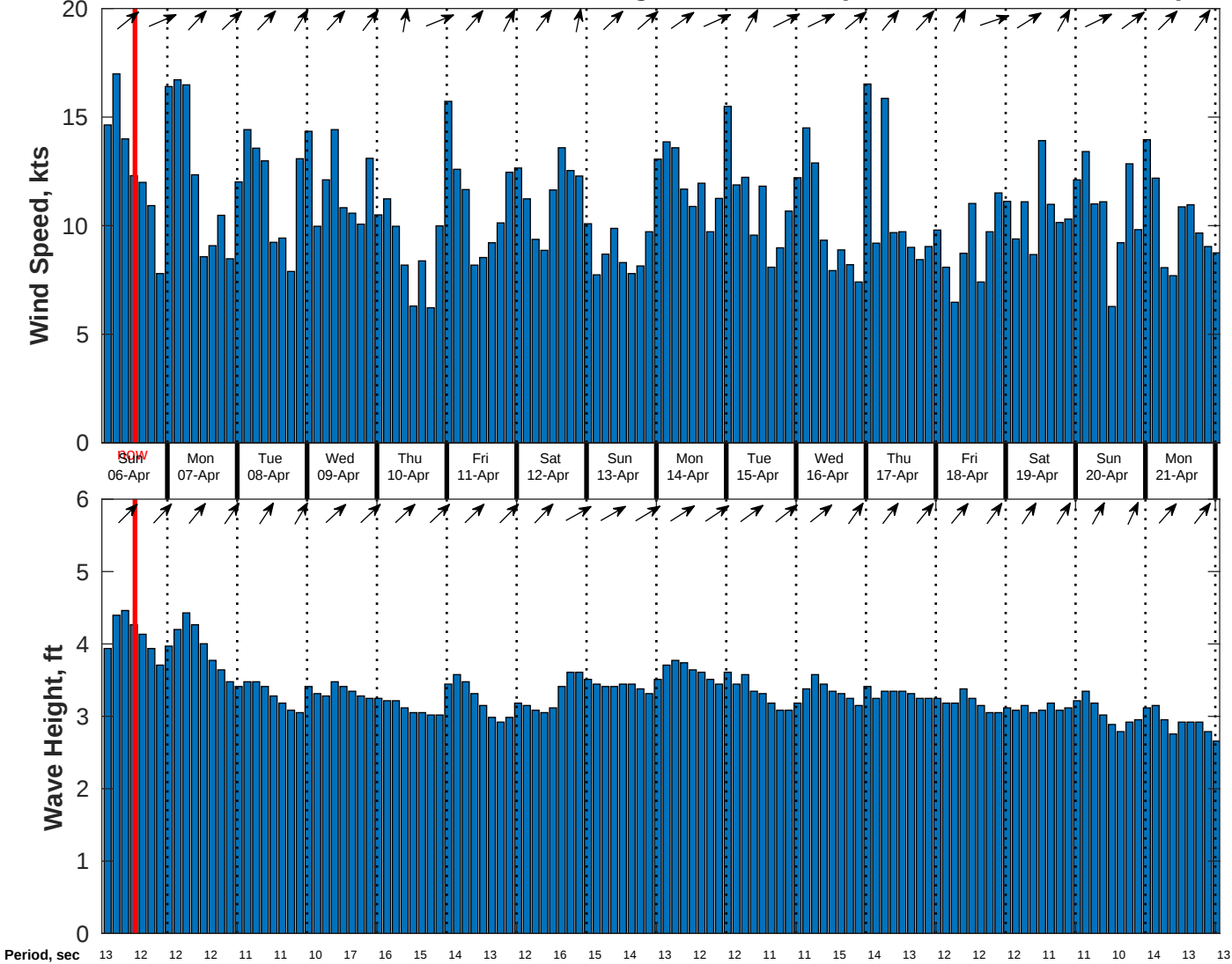
Wind & Wave Forecast for CSA (ONHYM) PPL EBS - Nigeria from 05-Apr-2025 02:00:00 to 21-Apr-2025 02:00:00
