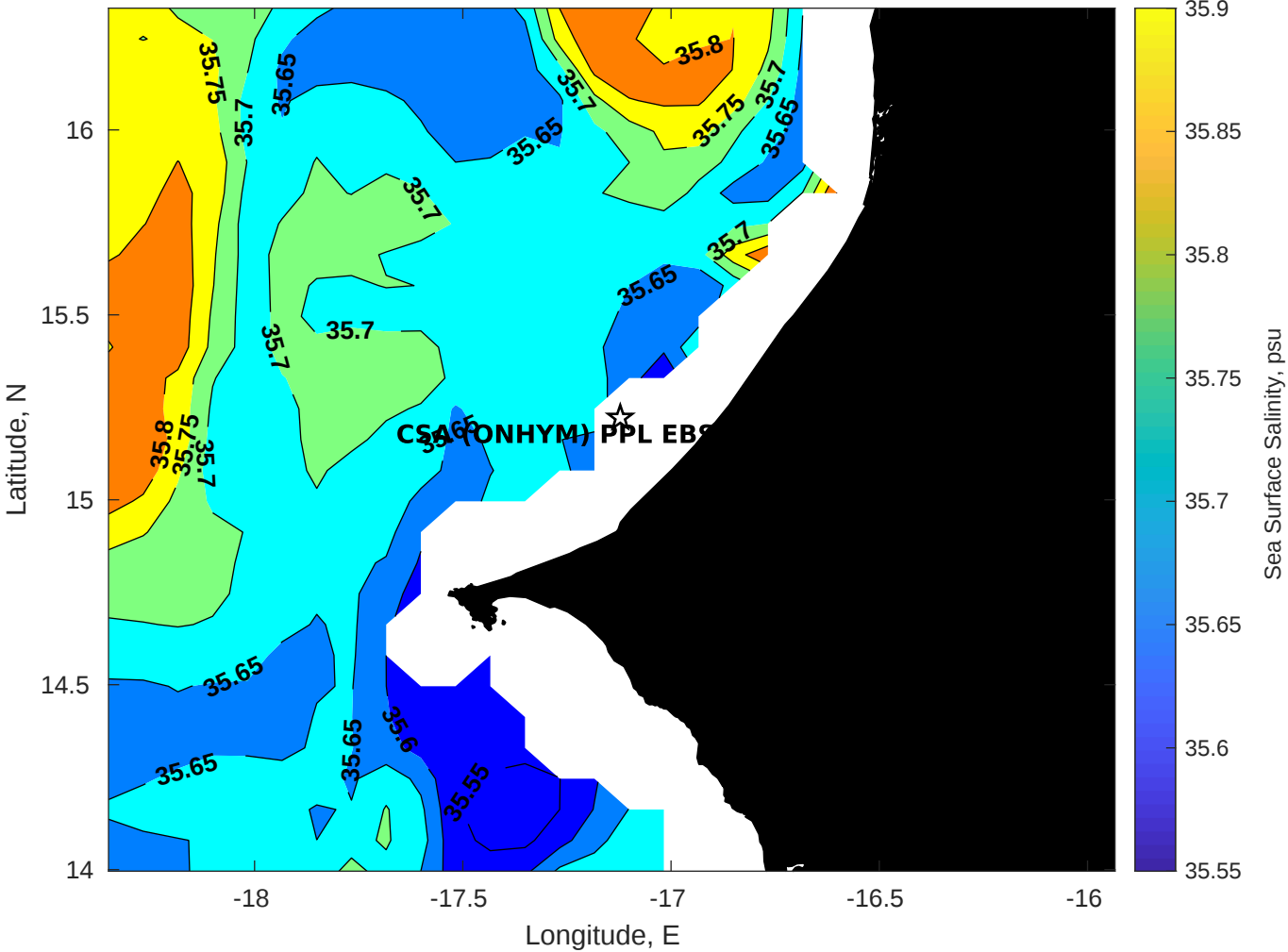
Surface Salinity for CSA (ONHYM) PPL EBS - Senegal at 04-Apr-2025 00:00:00
