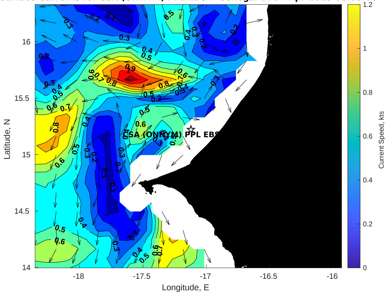
Surface Currents for CSA (ONHYM) PPL EBS - Senegal at 04-Apr-2025 00:00:00
