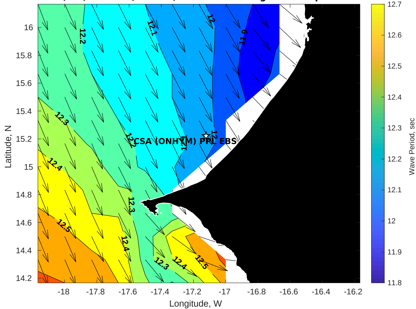
Wave Period (sec) for CSA (ONHYM) PPL EBS - Senegal at 05-Apr-2025 09:00:00
