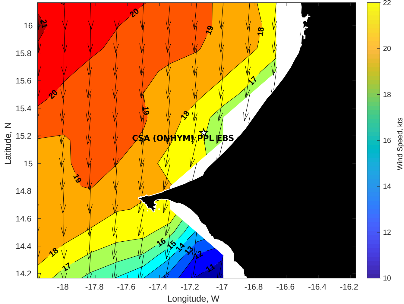
Winds (kts) for CSA (ONHYM) PPL EBS - Senegal at 05-Apr-2025 09:00:00
