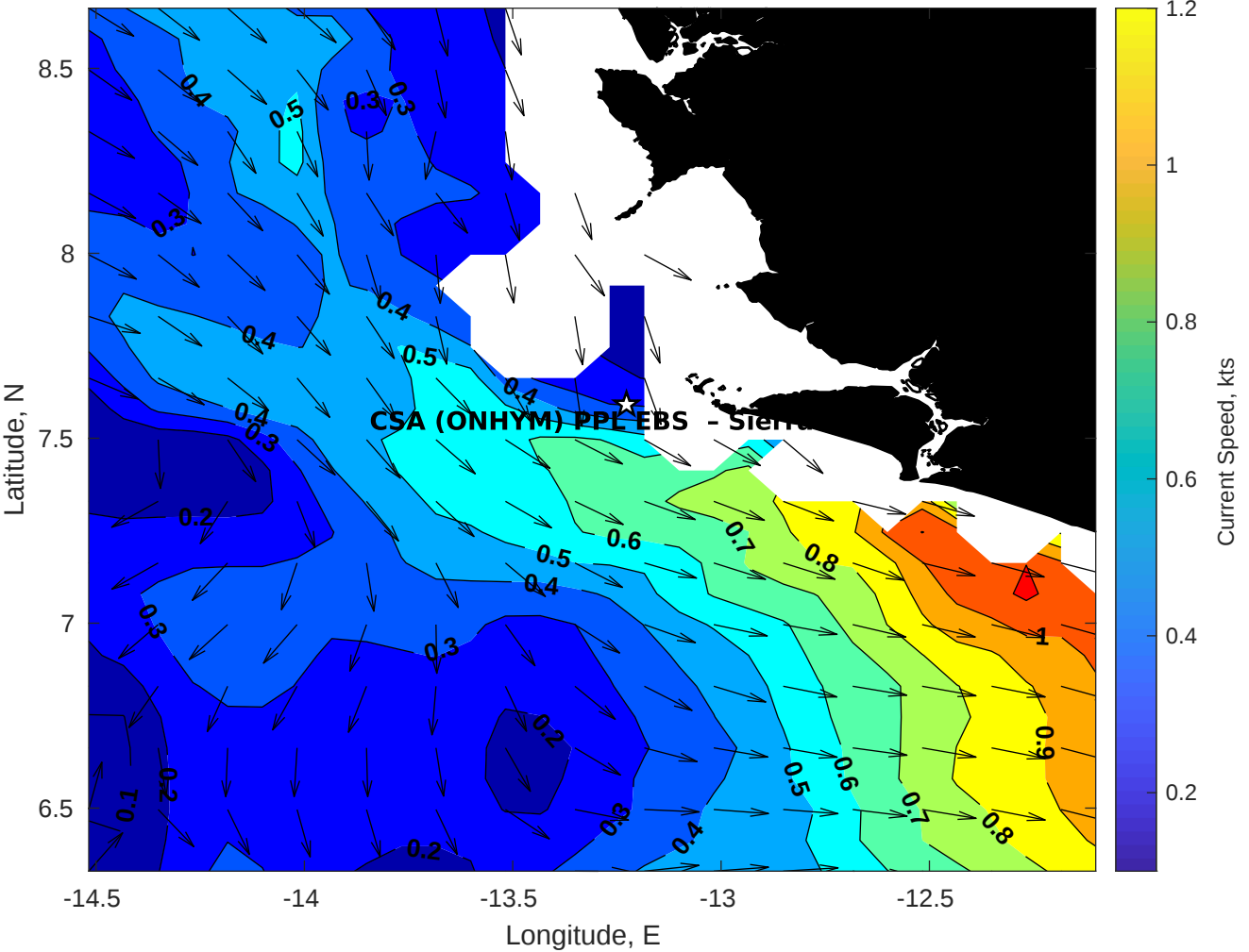
Surface Currents for CSA (ONHYM) PPL EBS - Sierra Leone at 04-Apr-2025 00:00:00
