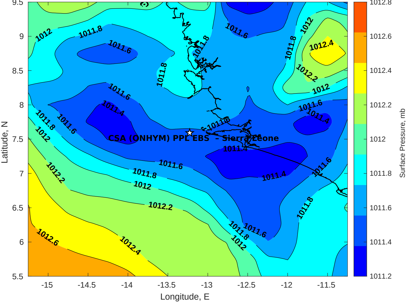
Surface Pressure (mb) for CSA (ONHYM) PPL EBS - Sierra Leone at 06-Apr-2025 00:00:00
