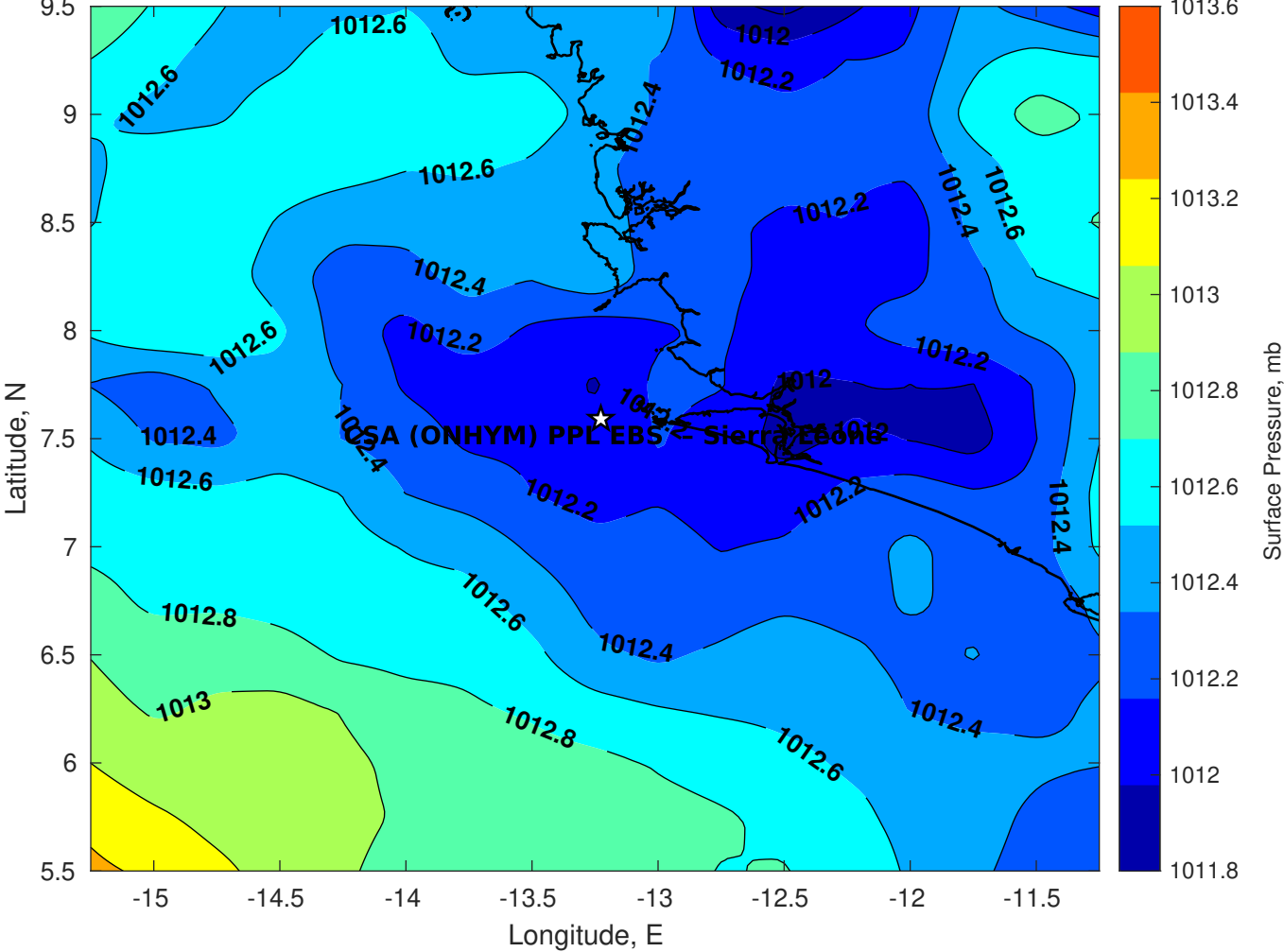
Surface Pressure (mb) for CSA (ONHYM) PPL EBS - Sierra Leone at 05-Apr-2025 00:00:00
