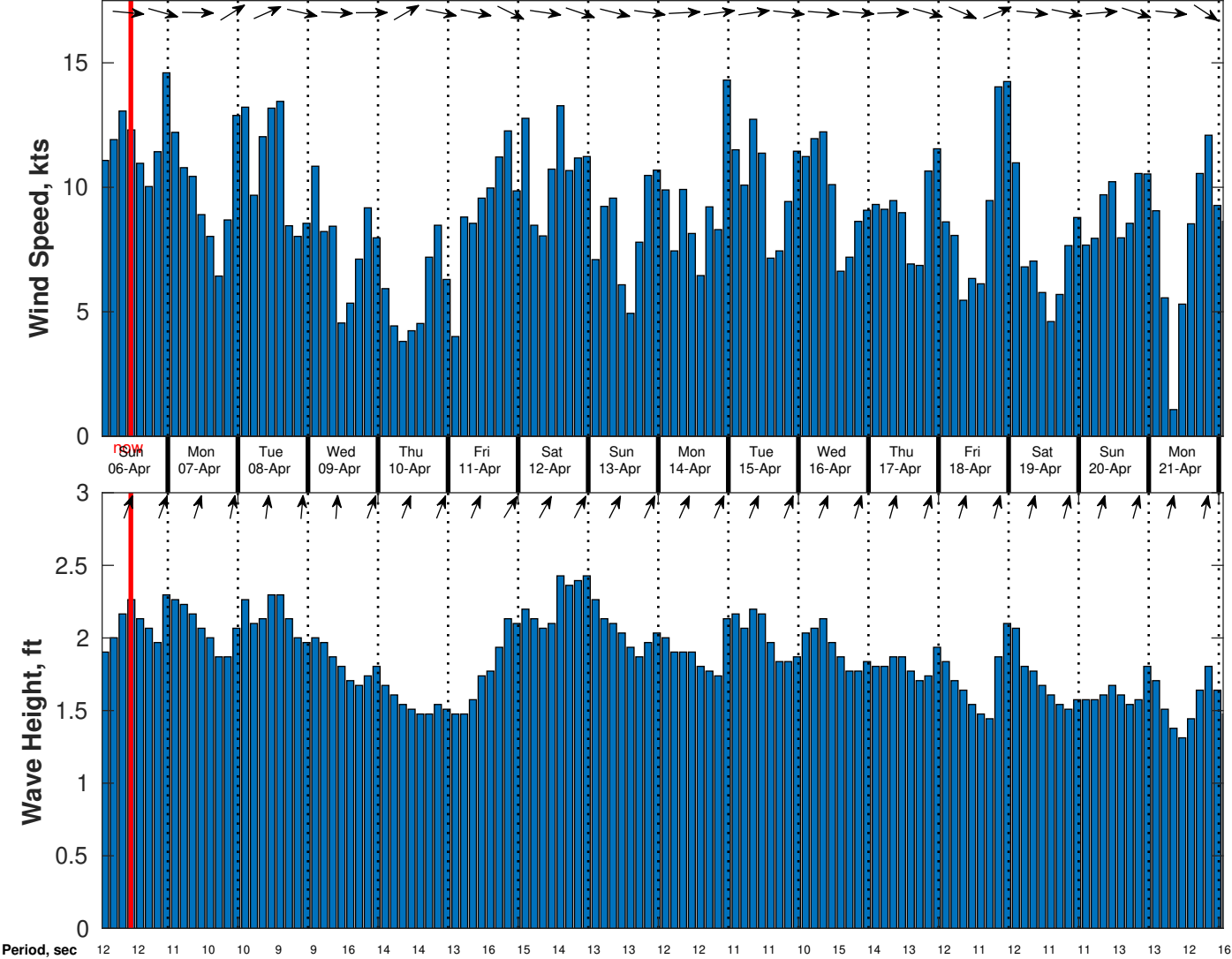
Wind & Wave Forecast for CSA (ONHYM) PPL EBS - Sierra Leone from 05-Apr-2025 01:00:00 to 21-Apr-2025 01:00:00
