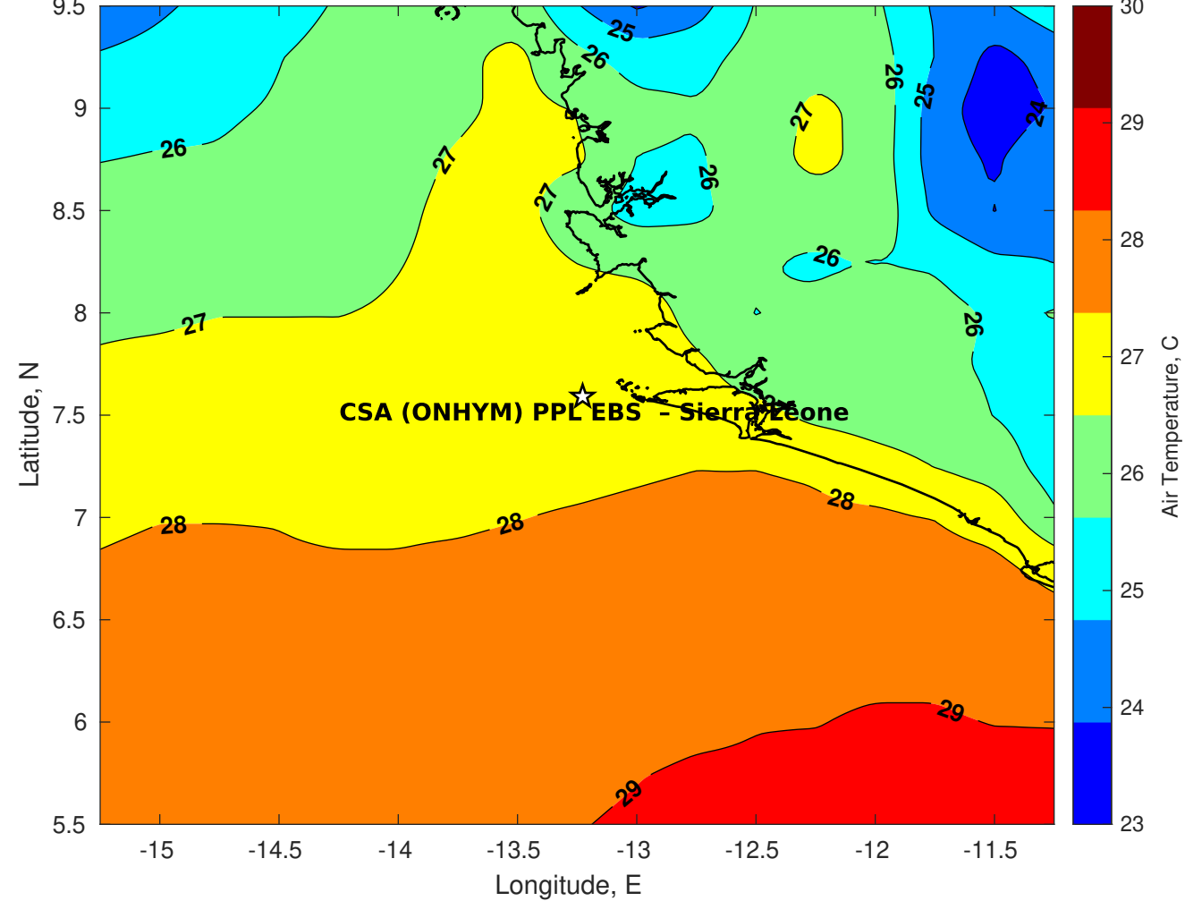
Air Temperature (C) for CSA (ONHYM) PPL EBS - Sierra Leone at 05-Apr-2025
