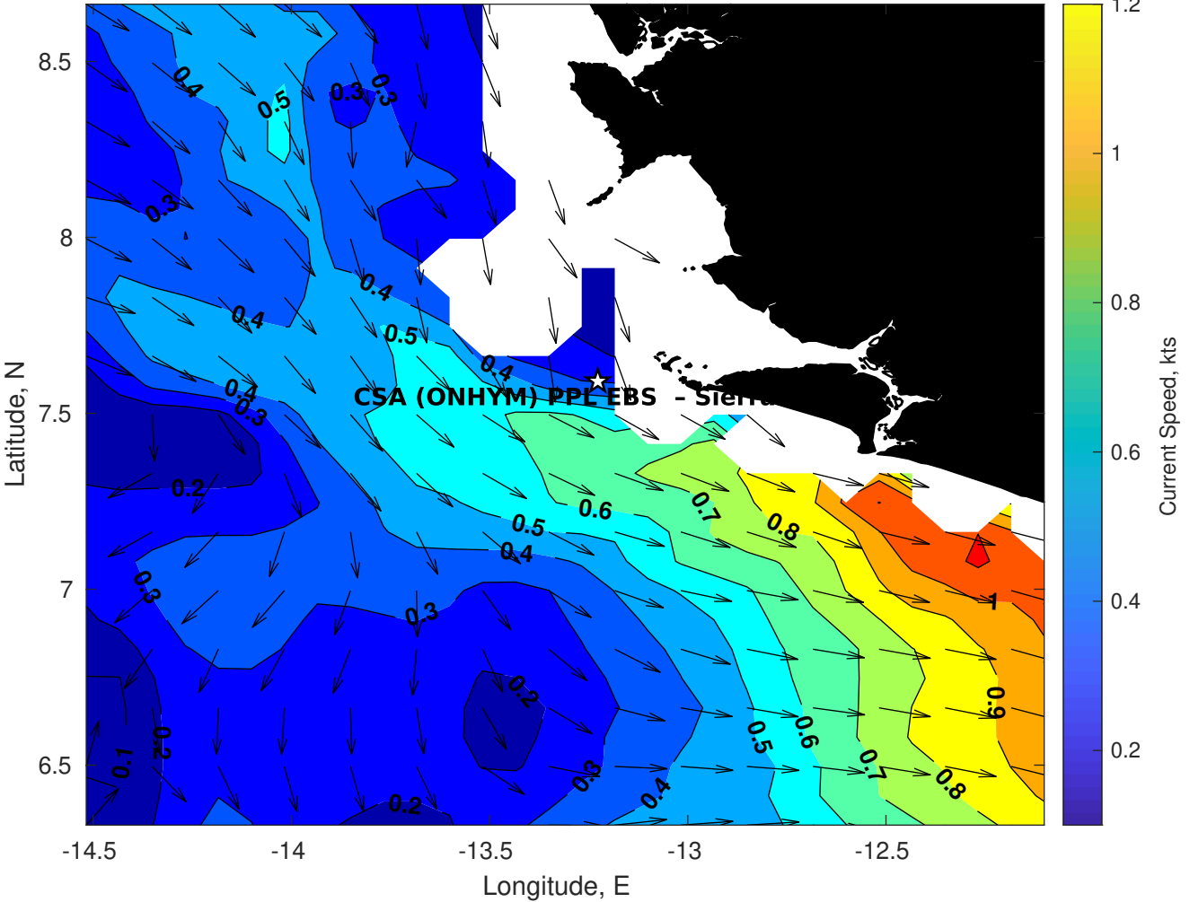
Surface Currents for CSA (ONHYM) PPL EBS - Sierra Leone at 04-Apr-2025 00:00:00
