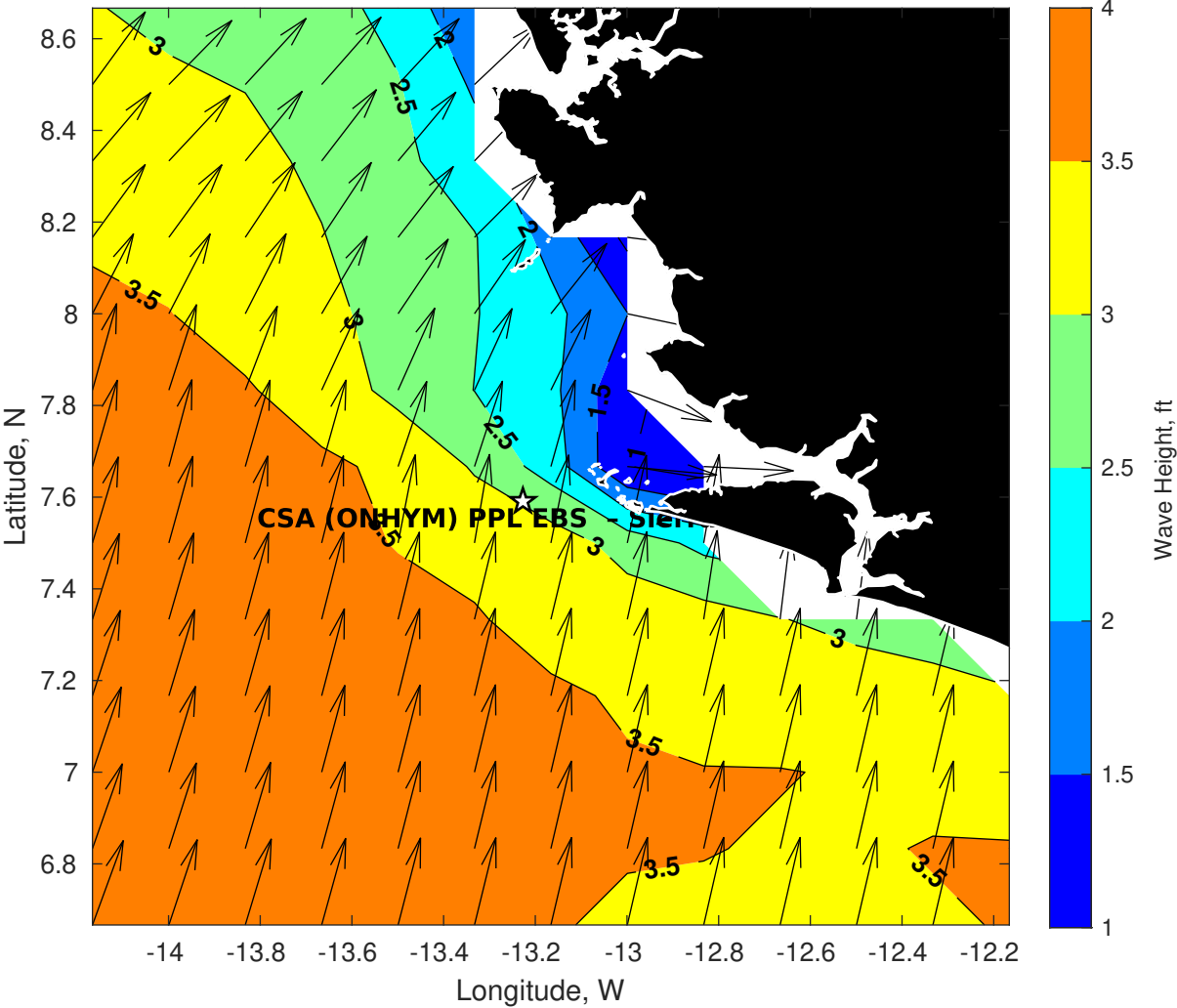
Wave Height (ft) for CSA (ONHYM) PPL EBS - Sierra Leone at 05-Apr-2025 09:00:00
