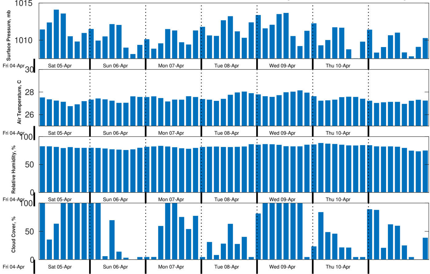
Met Forecast for CSA (ONHYM) PPL EBS - Sierra Leone from 05-Apr-2025 00:00:00 to 12-Apr-2025 00:00:00
