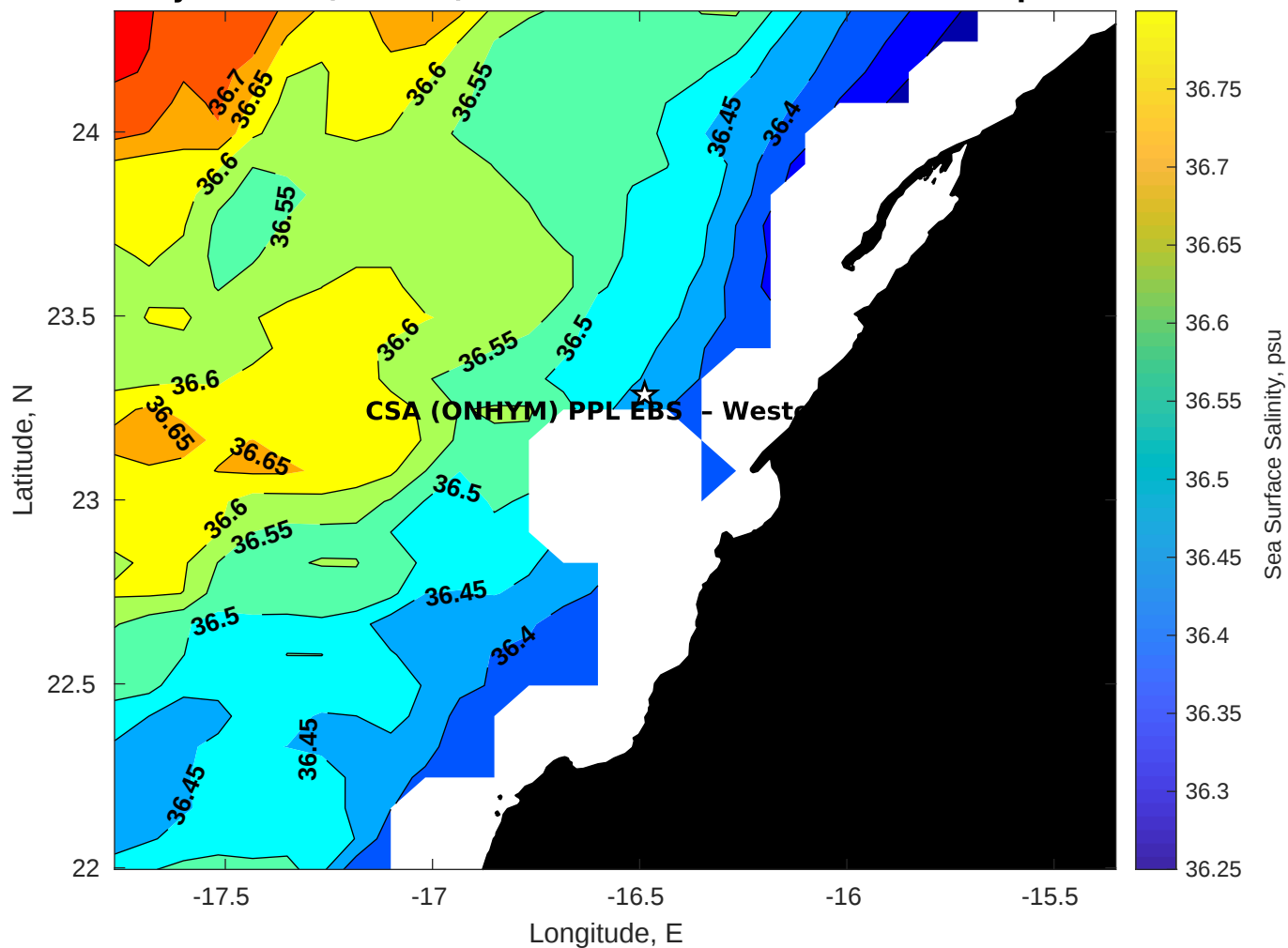
Surface Salinity for CSA (ONHYM) PPL EBS - Western Sahara at 04-Apr-2025 00:00:00
