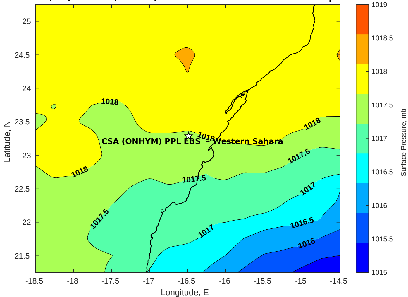
Surface Pressure (mb) for CSA (ONHYM) PPL EBS - Western Sahara at 06-Apr-2025 00:00:00
