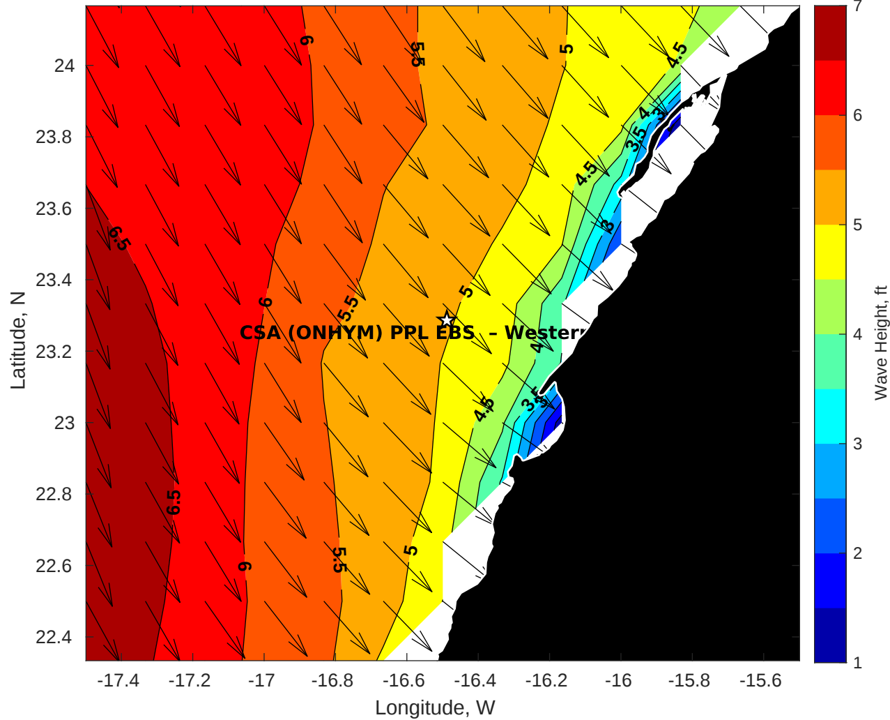
Wave Height (ft) for CSA (ONHYM) PPL EBS - Western Sahara at 05-Apr-2025 09:00:00
