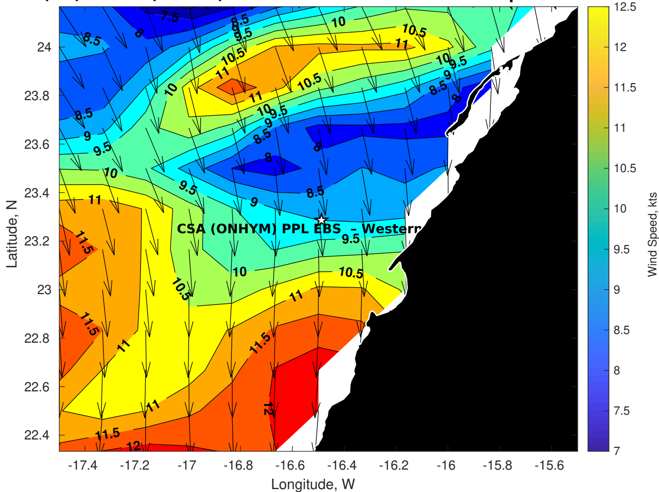
Winds (kts) for CSA (ONHYM) PPL EBS - Western Sahara at 05-Apr-2025 09:00:00
