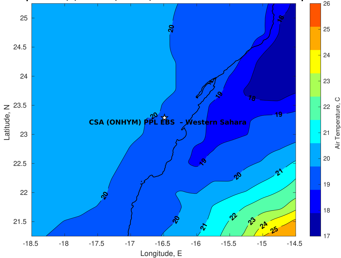
Air Temperature (C) for CSA (ONHYM) PPL EBS - Western Sahara at 05-Apr-2025
