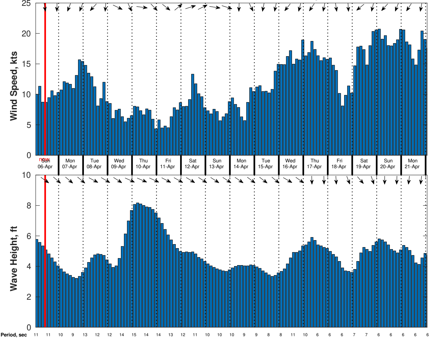
Wind & Wave Forecast for CSA (ONHYM) PPL EBS - Western Sahara from 05-Apr-2025 01:00:00 to 21-Apr-2025 01:00:00
