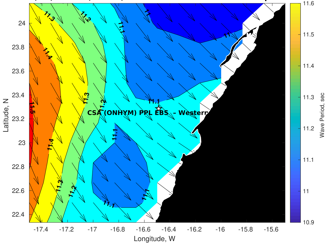
Wave Period (sec) for CSA (ONHYM) PPL EBS - Western Sahara at 05-Apr-2025 09:00:00
