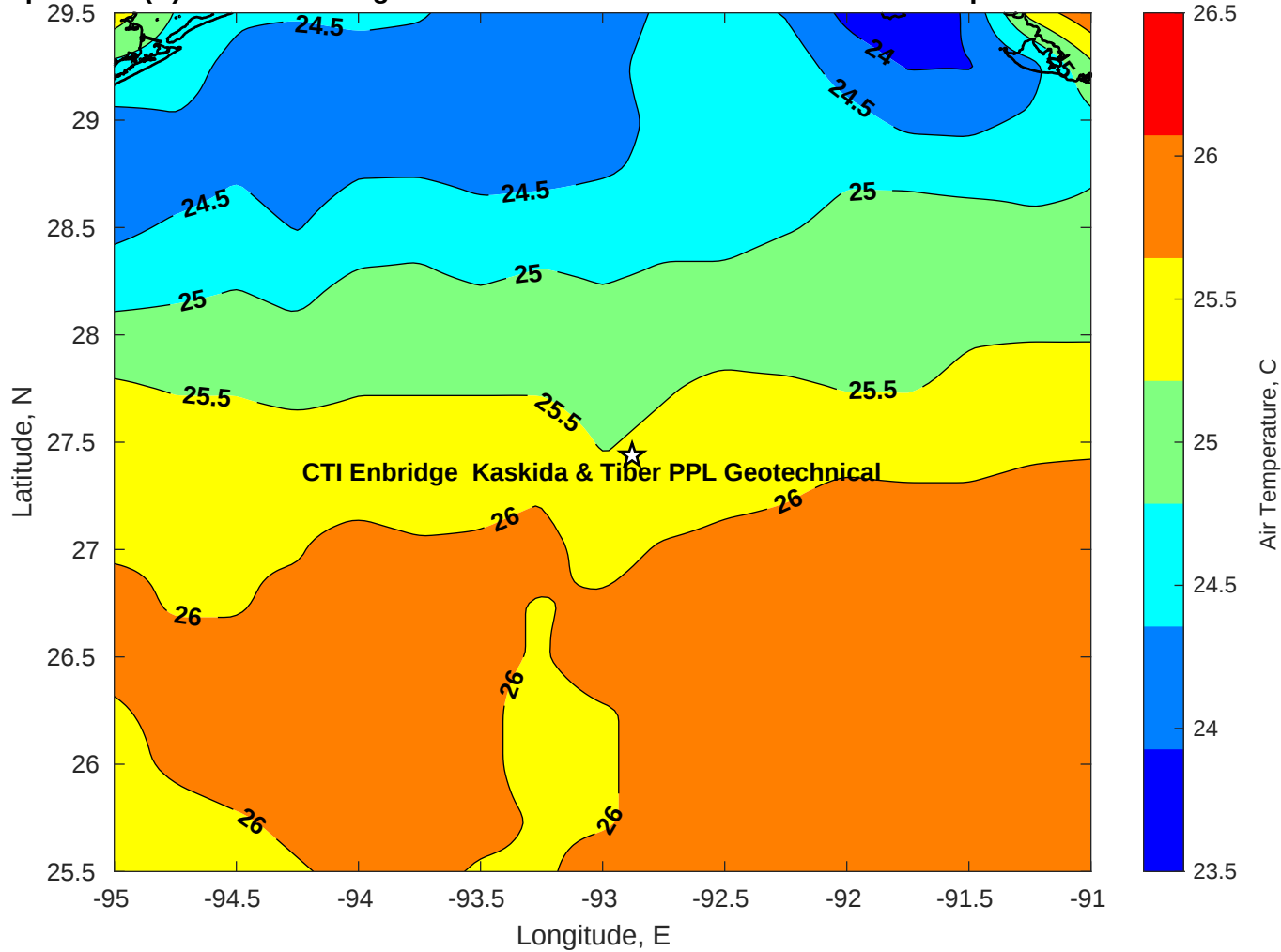
Air Temperature (C) for CTI Enbridge Kaskida & Tiber PPL Geotechnical at 05-Apr-2025
