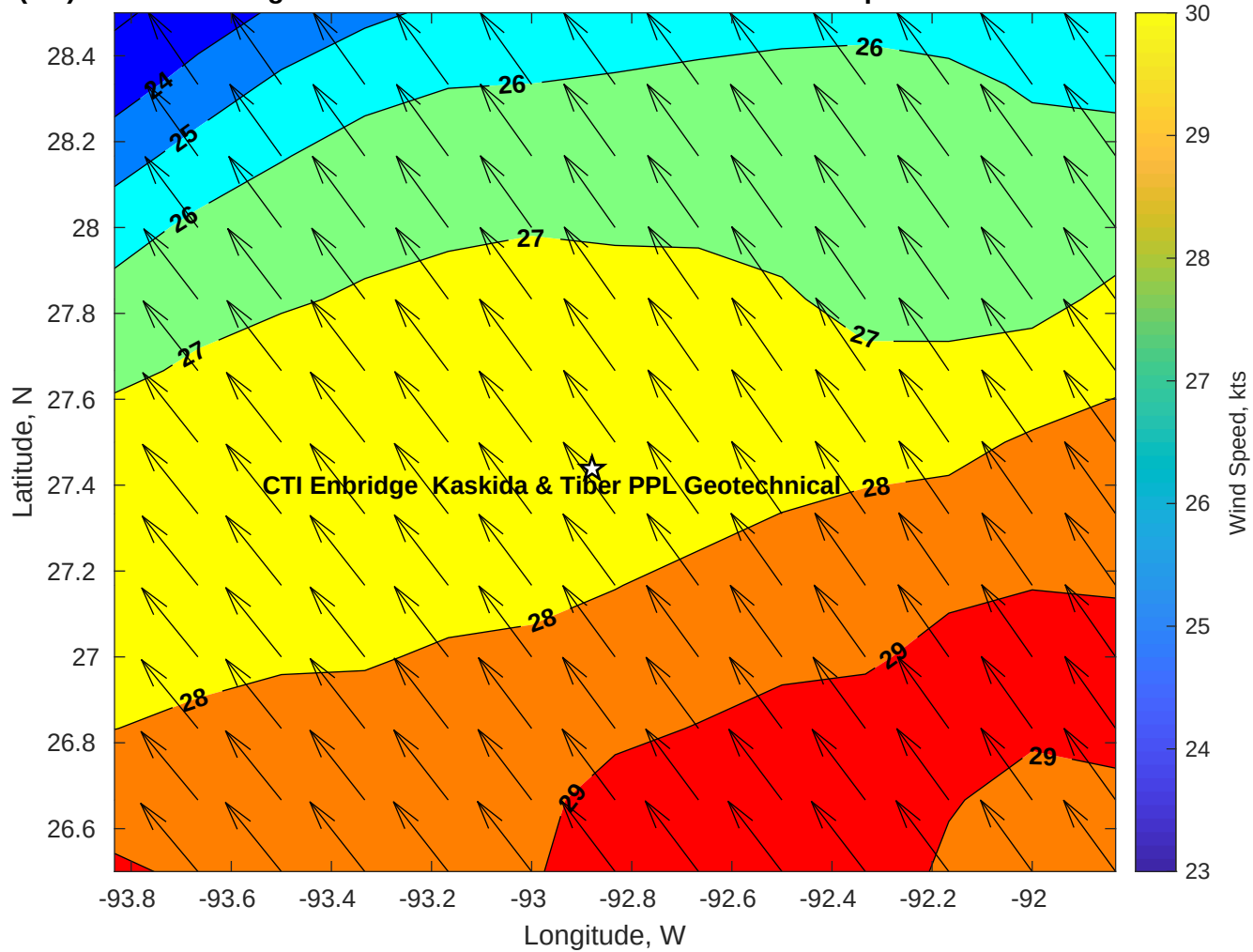
Winds (kts) for CTI Enbridge Kaskida & Tiber PPL Geotechnical at 05-Apr-2025 09:00:00
