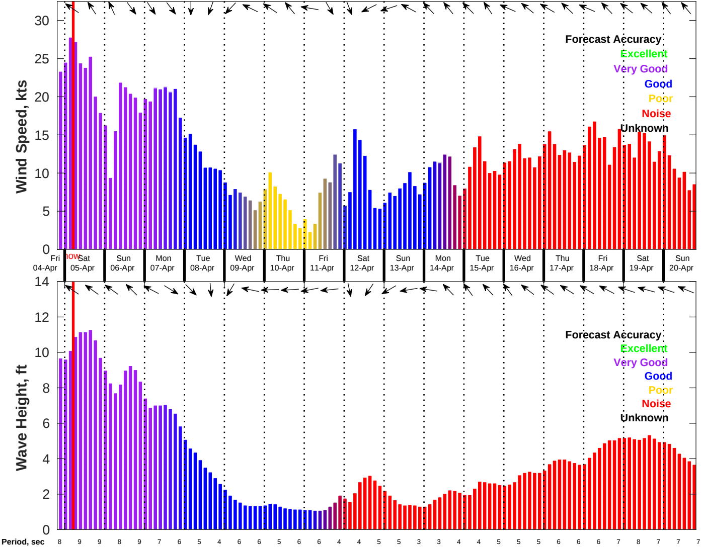
Wind & Wave Forecast for CTI Enbridge Kaskida & Tiber PPL Geotechnical from 04-Apr-2025 20:00:00 to 20-Apr-2025 20:00:00
