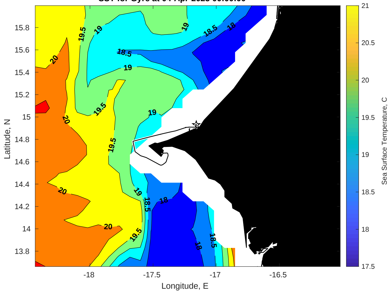
SST for Gyre at 04-Apr-2025 00:00:00
