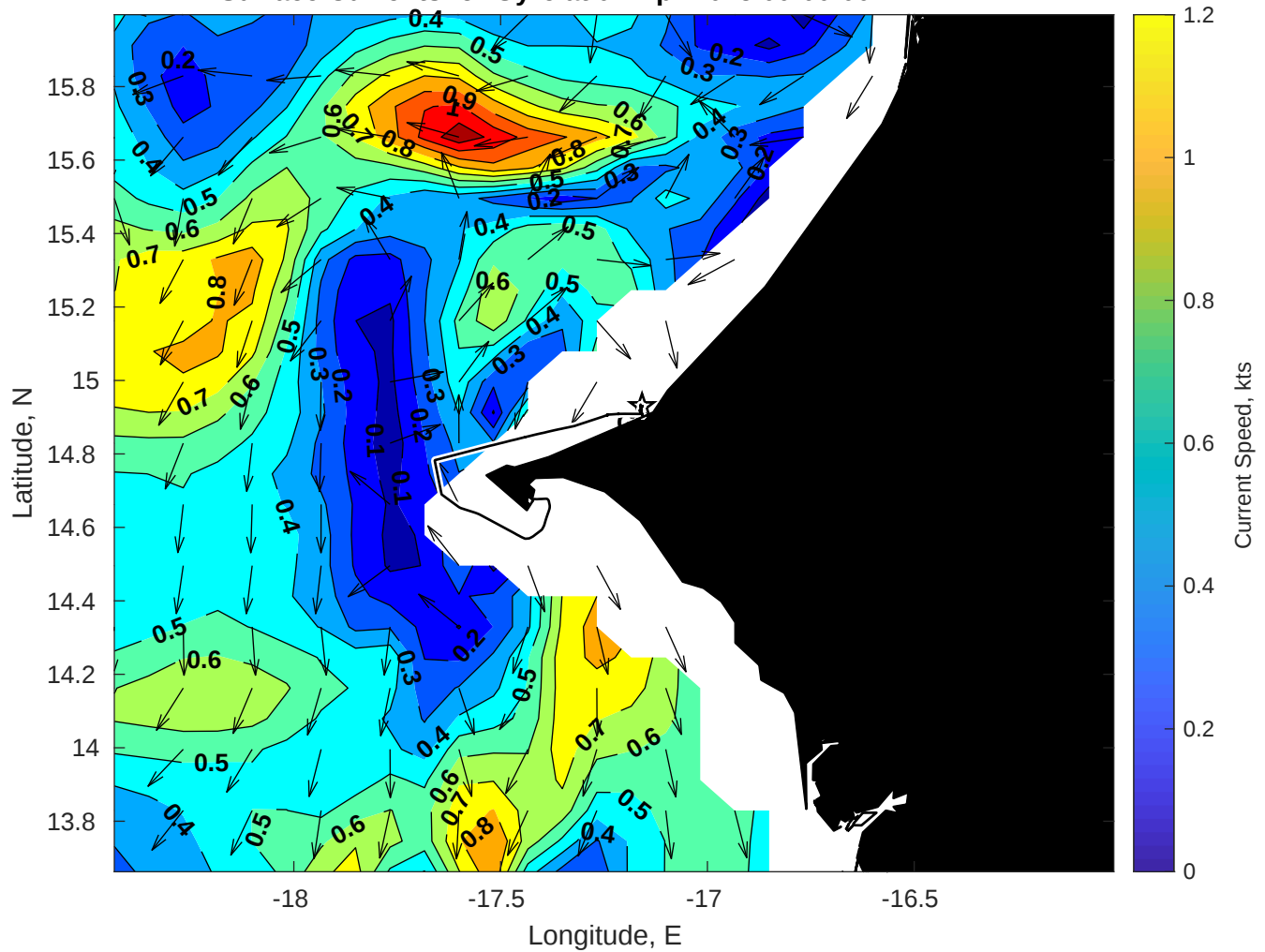
Surface Currents for Gyre at 04-Apr-2025 00:00:00
