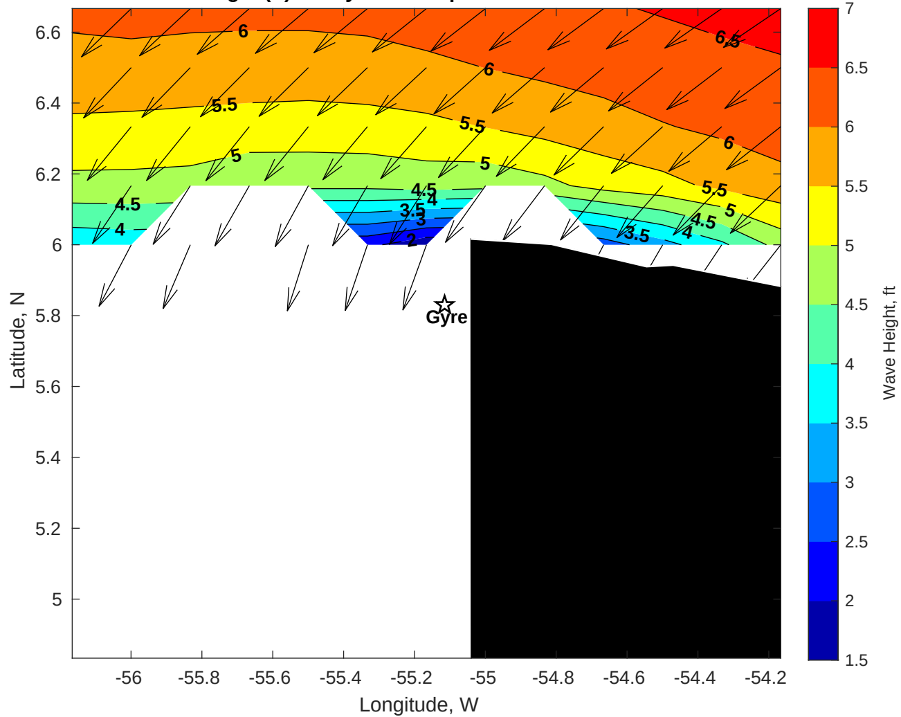
Wave Height (ft) for Gyre at 05-Apr-2025 09:00:00
