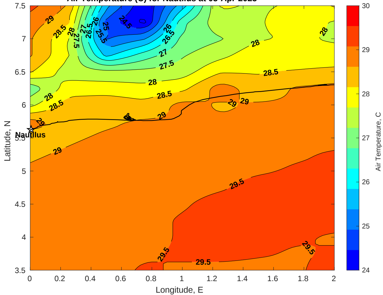
Air Temperature (C) for Nautilus at 05-Apr-2025
