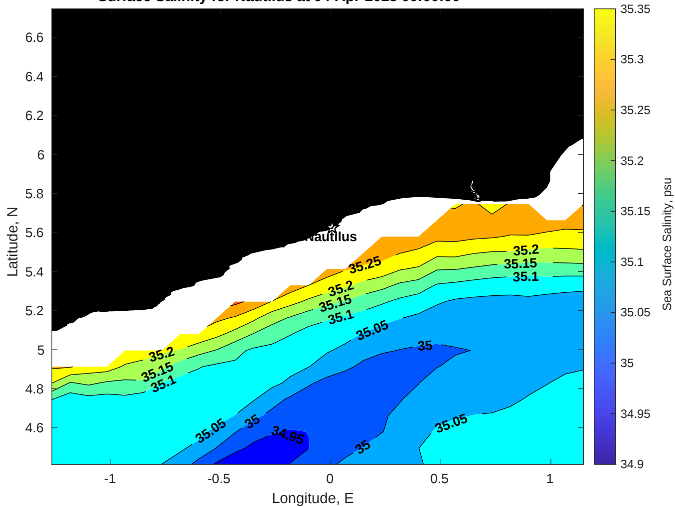
Surface Salinity for Nautilus at 04-Apr-2025 00:00:00
