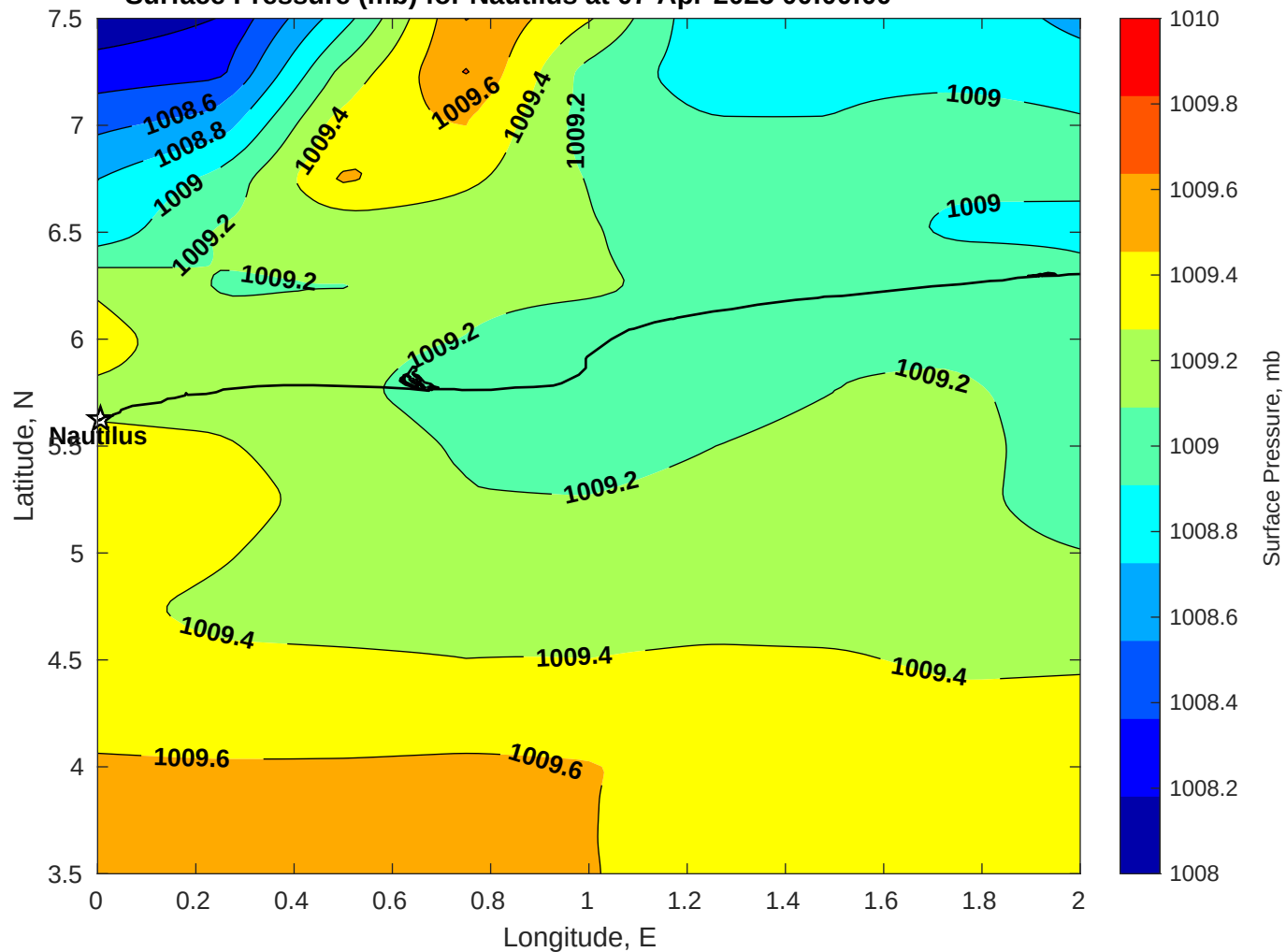
Surface Pressure (mb) for Nautilus at 07-Apr-2025 00:00:00
