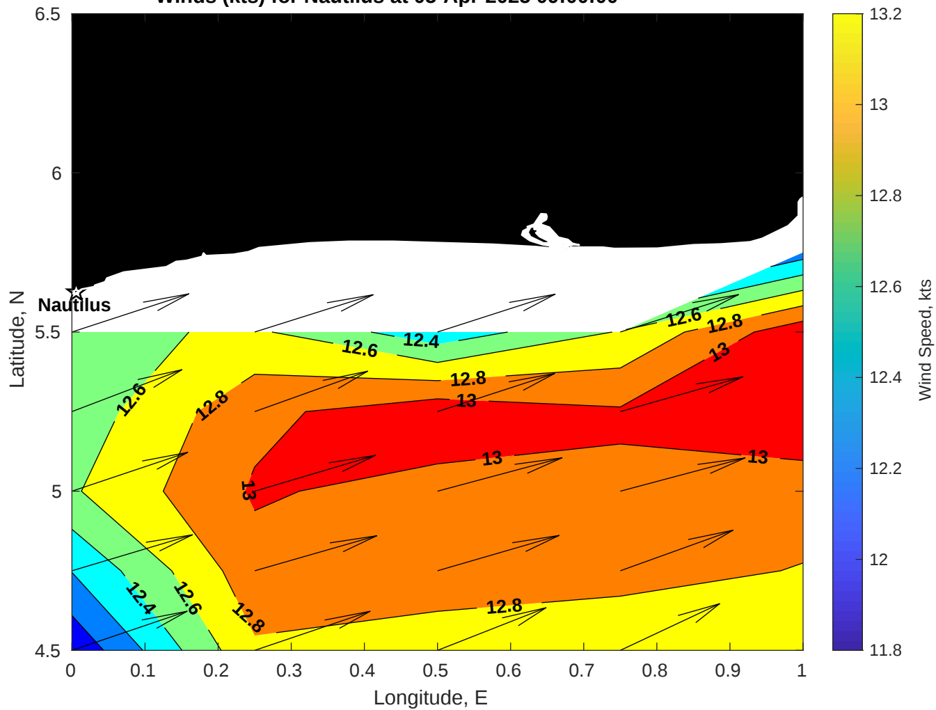
Winds (kts) for Nautilus at 05-Apr-2025 09:00:00
