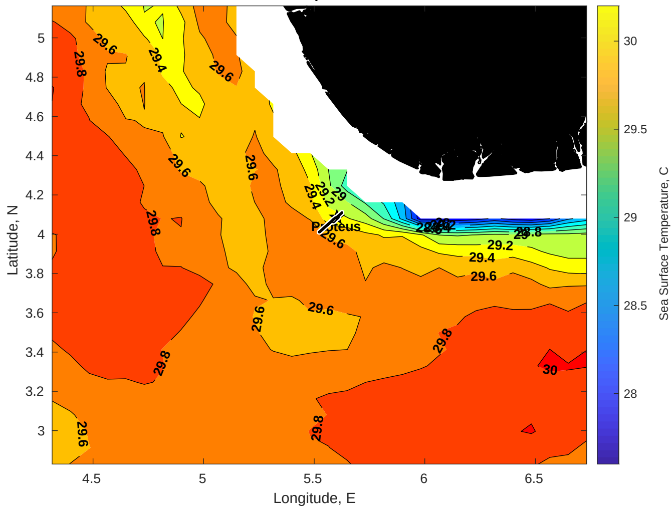
SST for Proteus at 04-Apr-2025 00:00:00
