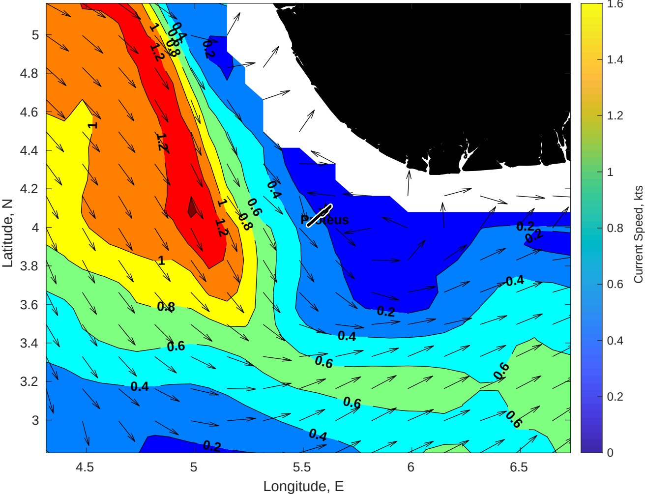
Surface Currents for Proteus at 04-Apr-2025 00:00:00
