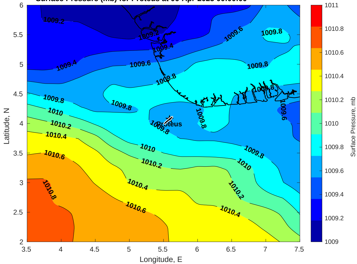
Surface Pressure (mb) for Proteus at 06-Apr-2025 00:00:00
