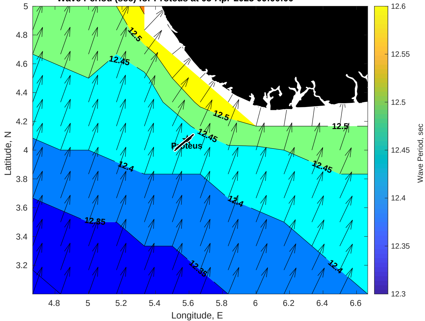
Wave Period (sec) for Proteus at 05-Apr-2025 09:00:00
