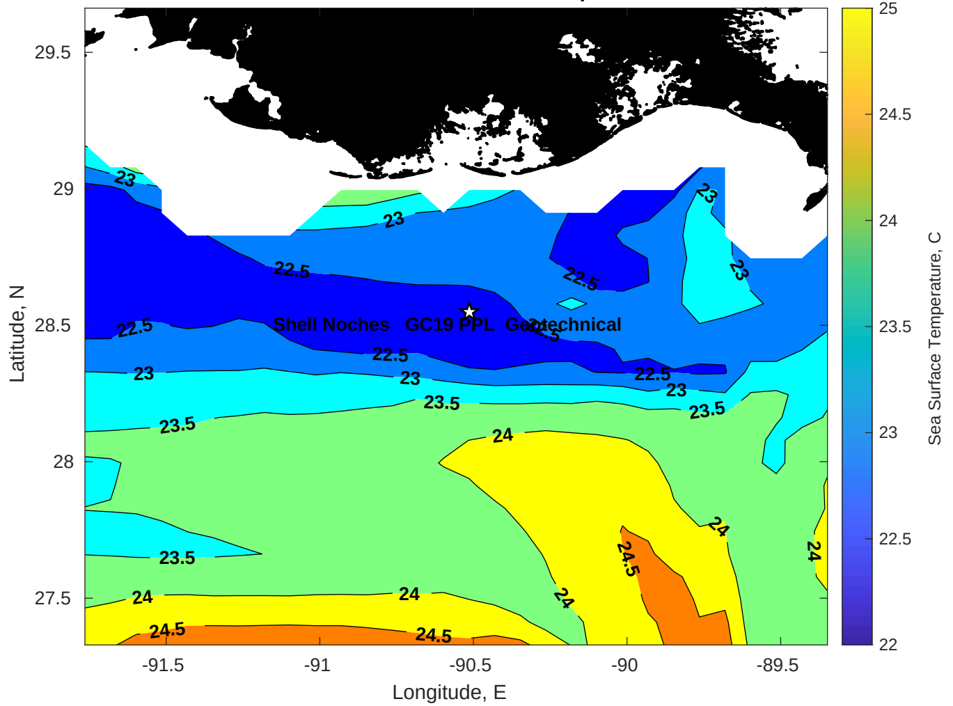
SST for Shell Noches GC19 PPL Geotechnical at 04-Apr-2025 00:00:00
