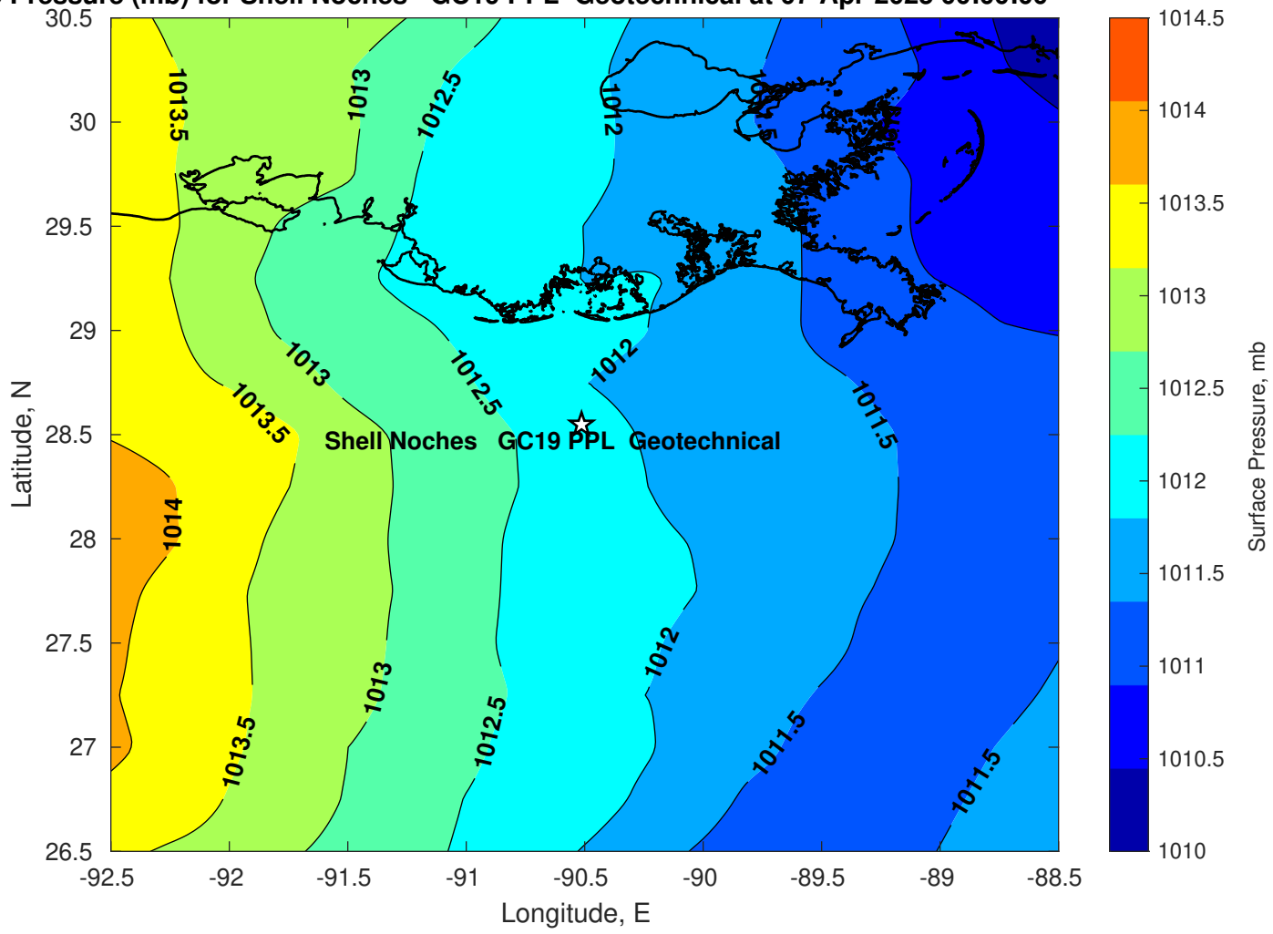
Surface Pressure (mb) for Shell Noches GC19 PPL Geotechnical at 07-Apr-2025 00:00:00
