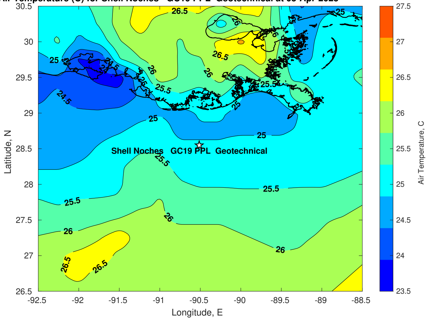
Air Temperature (C) for Shell Noches GC19 PPL Geotechnical at 05-Apr-2025
