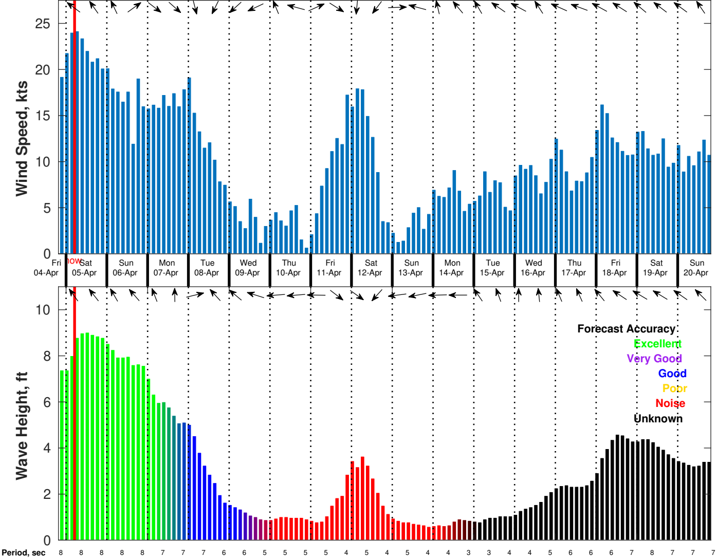
Wind & Wave Forecast for Shell Noches GC19 PPL Geotechnical from 04-Apr-2025 20:00:00 to 20-Apr-2025 20:00:00
