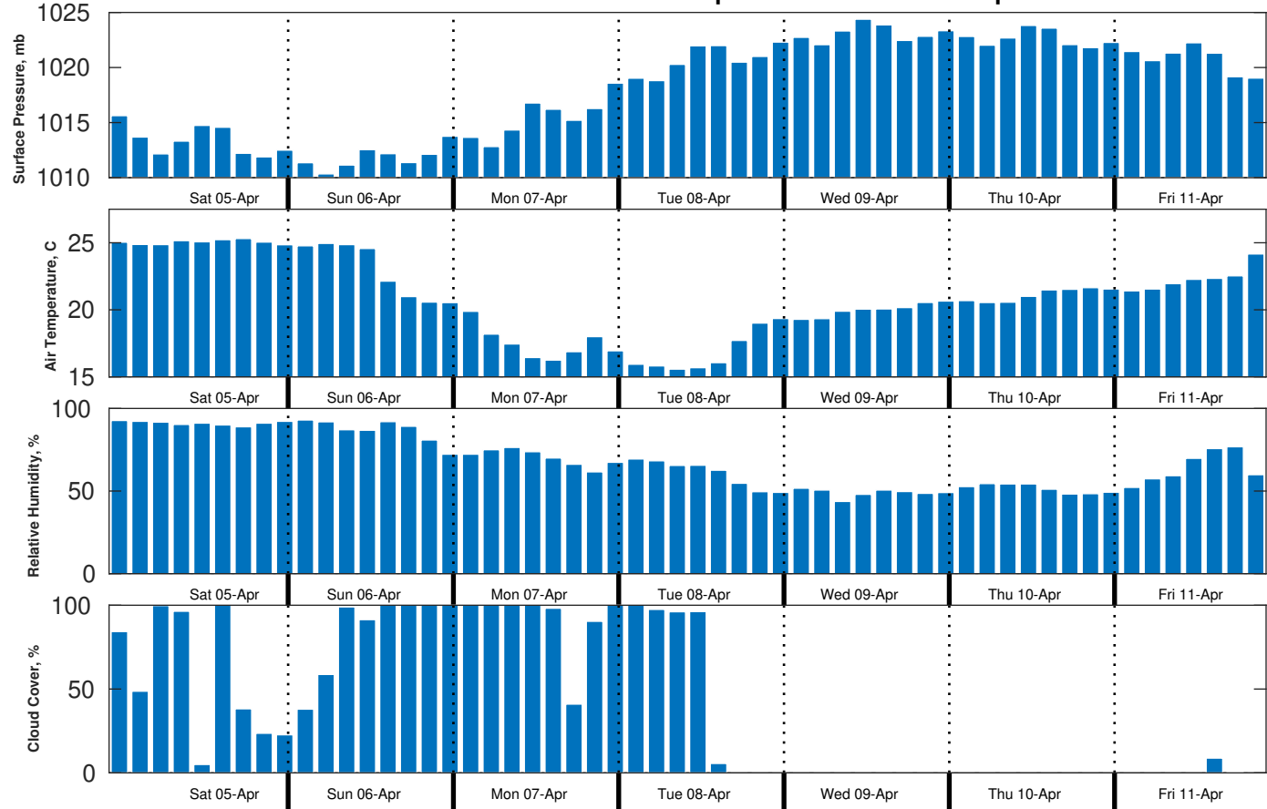
Met Forecast for Shell Noches GC19 PPL Geotechnical from 05-Apr-2025 00:00:00 to 12-Apr-2025 00:00:00
