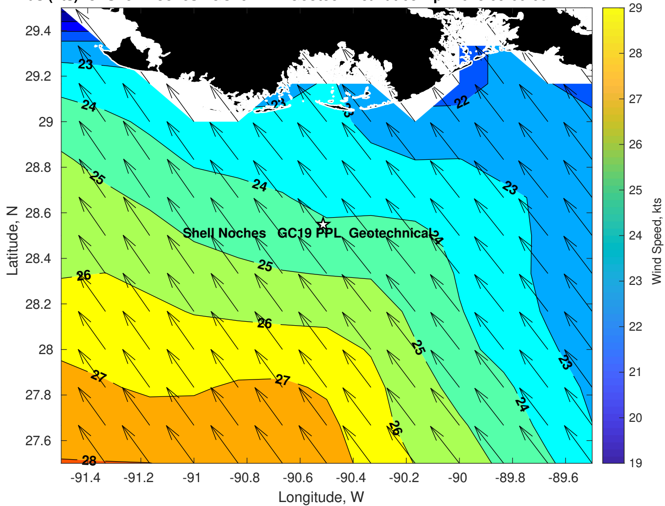
Winds (kts) for Shell Noches GC19 PPL Geotechnical at 05-Apr-2025 09:00:00
