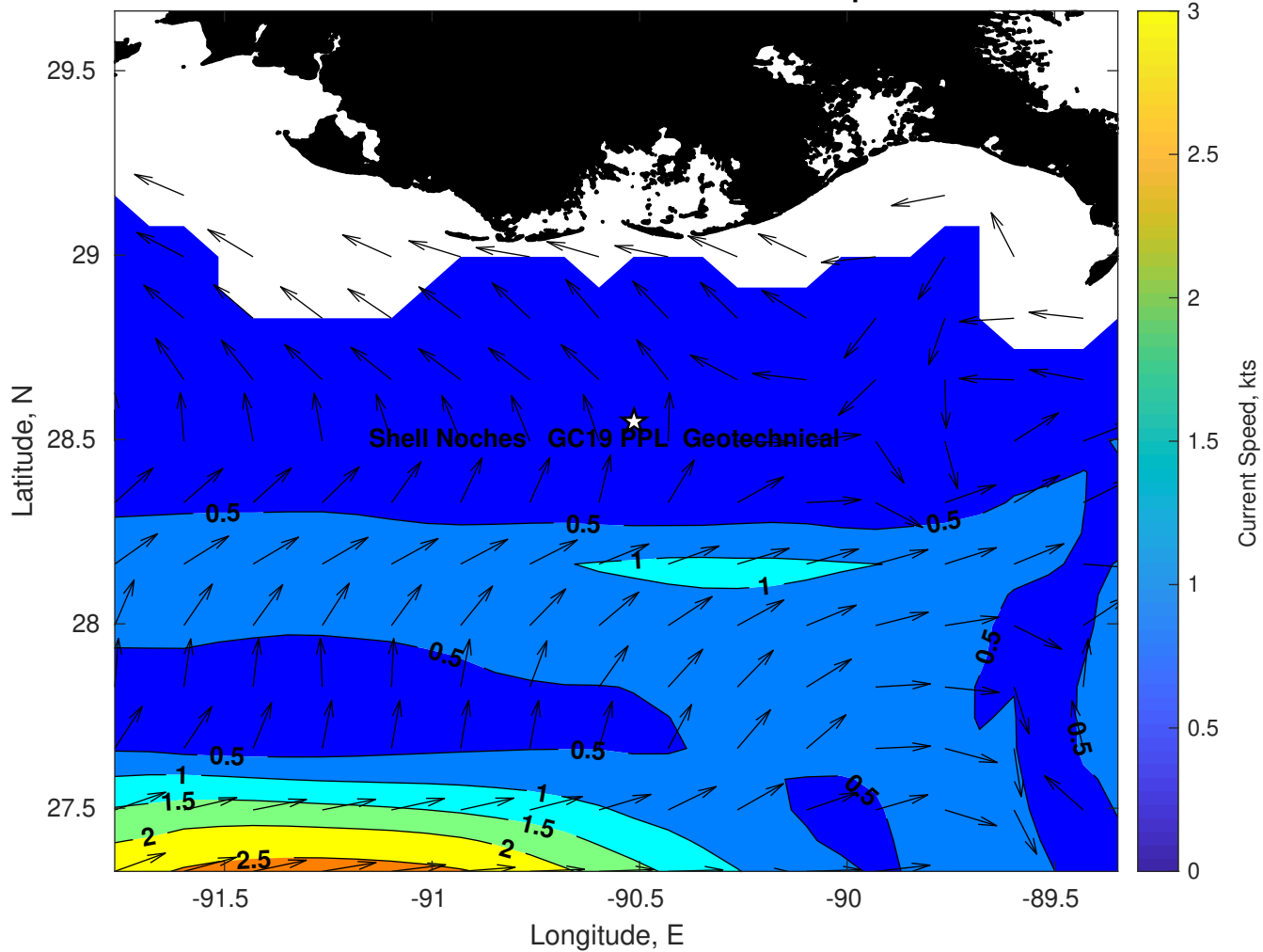
Surface Currents for Shell Noches GC19 PPL Geotechnical at 04-Apr-2025 00:00:00
