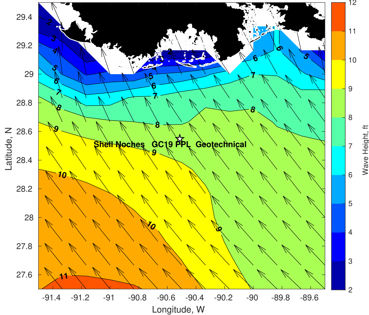
Wave Height (ft) for Shell Noches GC19 PPL Geotechnical at 05-Apr-2025 09:00:00
