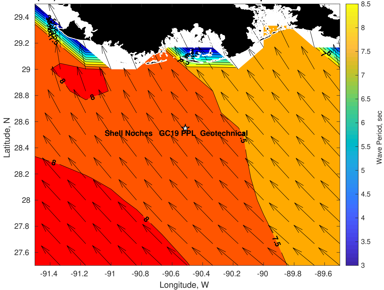
Wave Period (sec) for Shell Noches GC19 PPL Geotechnical at 05-Apr-2025 09:00:00
