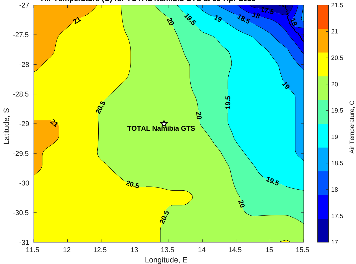
Air Temperature (C) for TOTAL Namibia GTS at 05-Apr-2025
