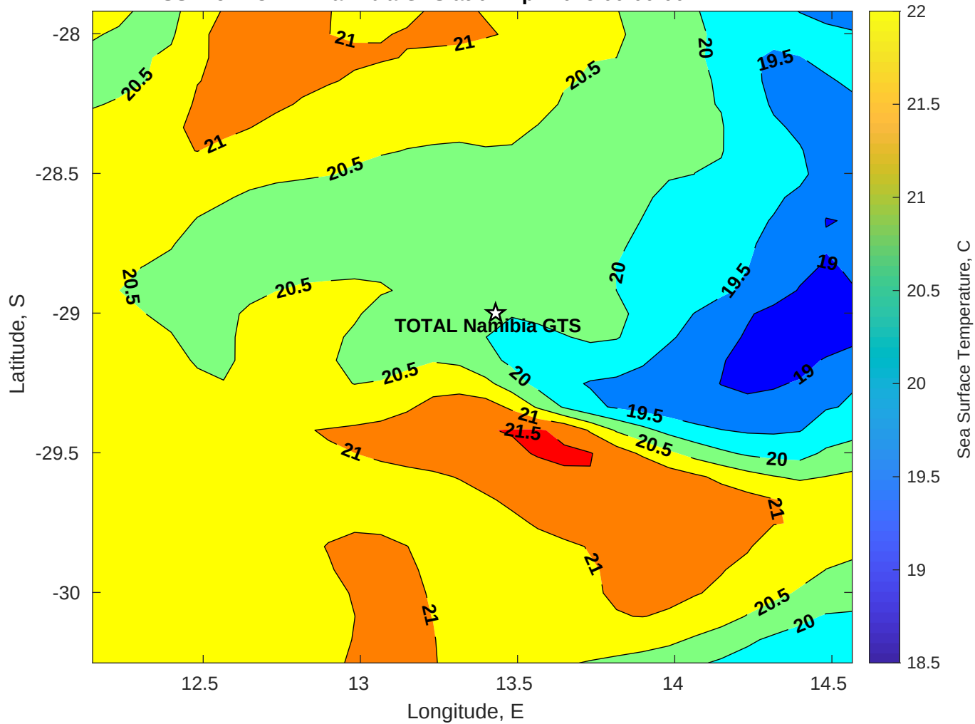
SST for TOTAL Namibia GTS at 04-Apr-2025 00:00:00
