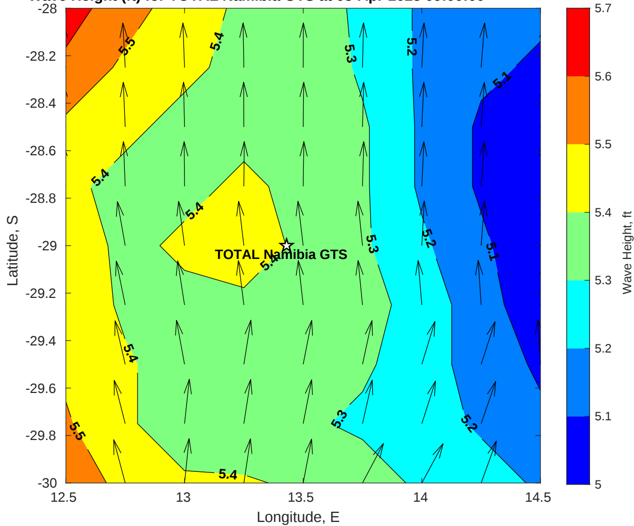
Wave Height (ft) for TOTAL Namibia GTS at 05-Apr-2025 09:00:00
