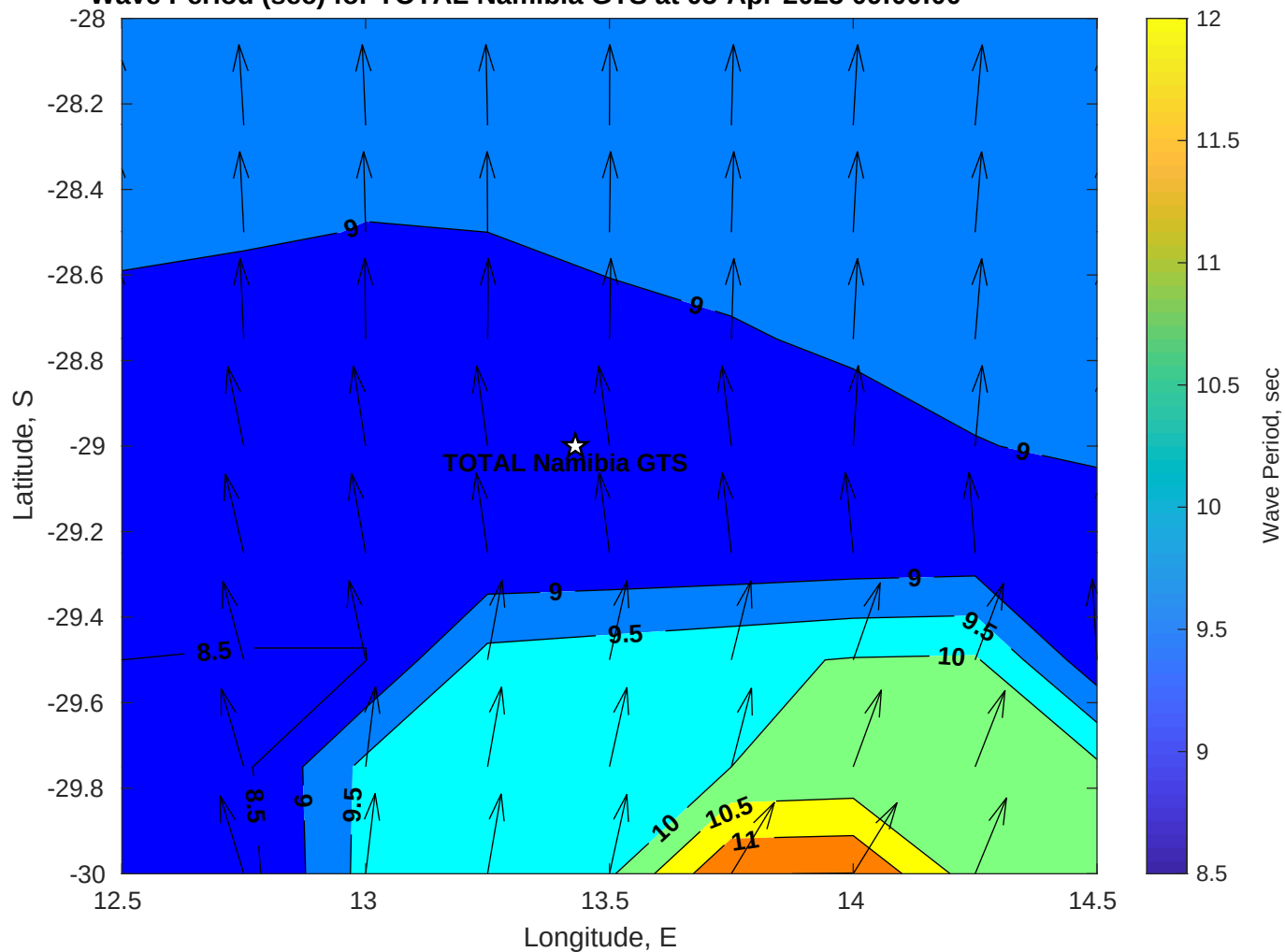
Wave Period (sec) for TOTAL Namibia GTS at 05-Apr-2025 09:00:00
