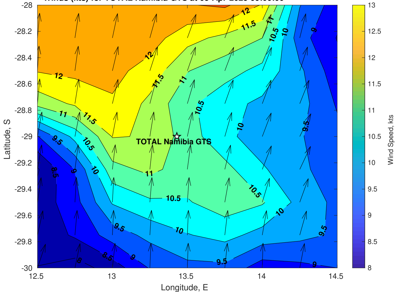
Winds (kts) for TOTAL Namibia GTS at 05-Apr-2025 09:00:00
