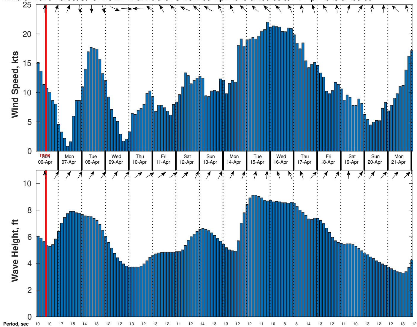
Wind & Wave Forecast for TOTAL Namibia GTS from 05-Apr-2025 02:00:00 to 21-Apr-2025 02:00:00
