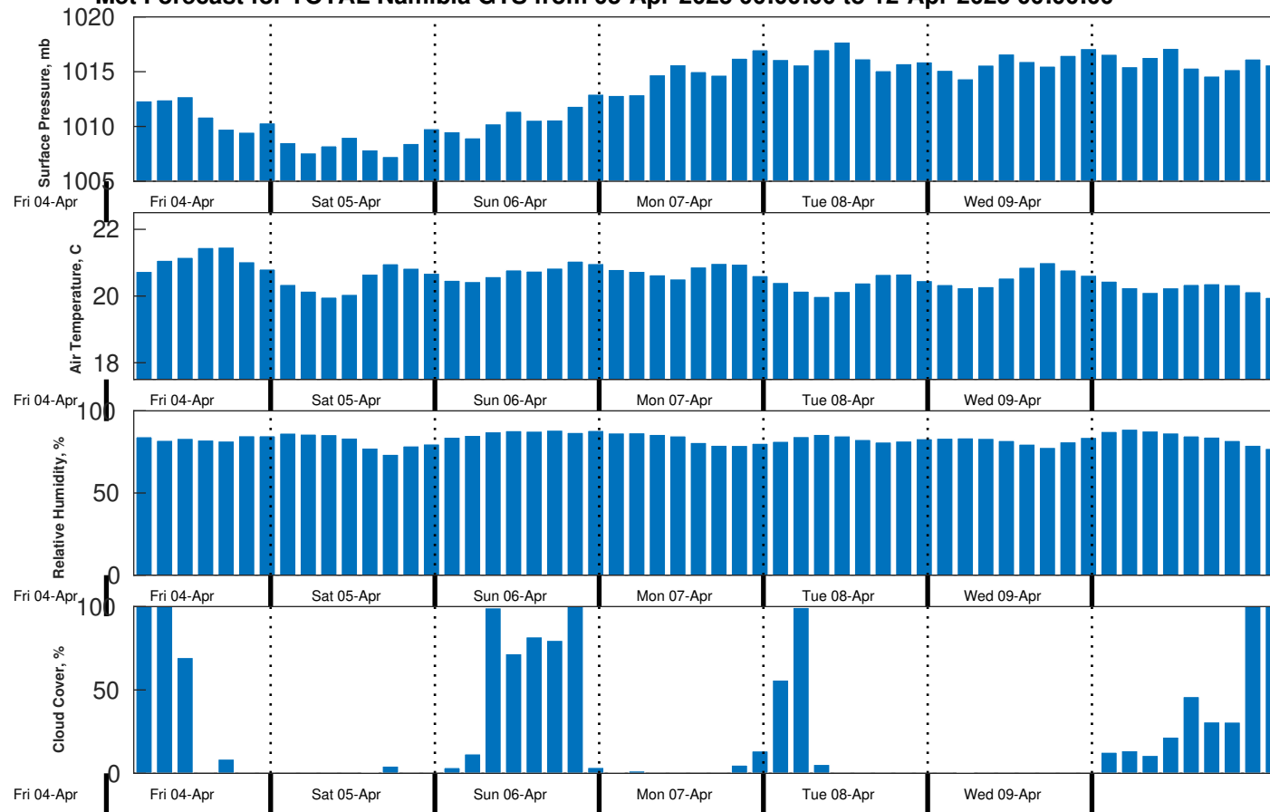
Met Forecast for TOTAL Namibia GTS from 05-Apr-2025 00:00:00 to 12-Apr-2025 00:00:00
