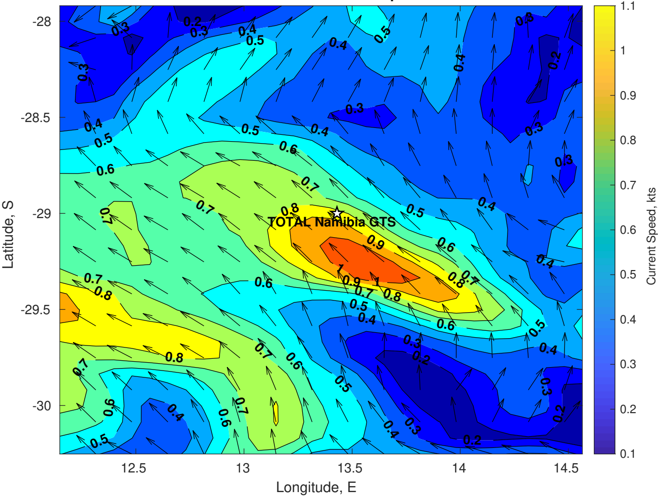
Surface Currents for TOTAL Namibia GTS at 04-Apr-2025 00:00:00
