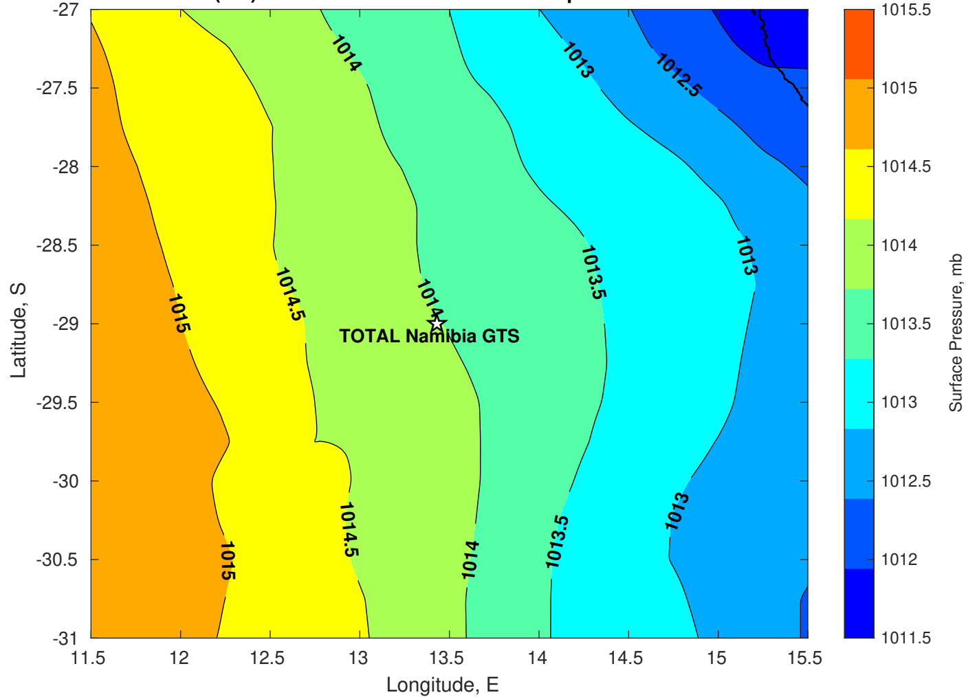
Surface Pressure (mb) for TOTAL Namibia GTS at 05-Apr-2025 00:00:00
