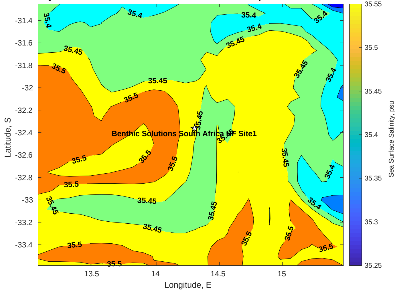
Surface Salinity for Benthic Solutions South Africa HF Site1 at 05-Apr-2025 00:00:00
