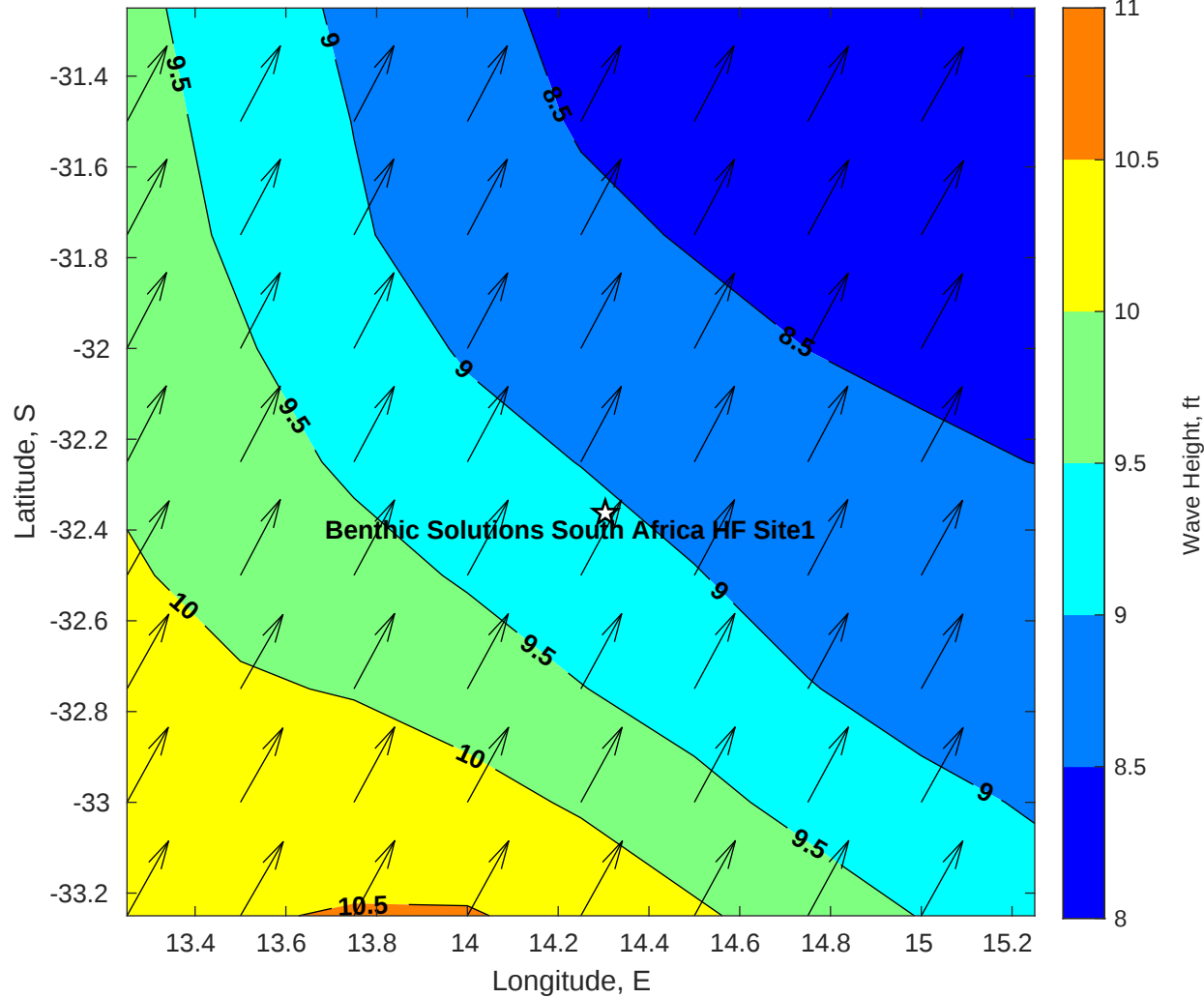
Wave Height (ft) for Benthic Solutions South Africa HF Site1 at 06-Apr-2025 09:00:00
