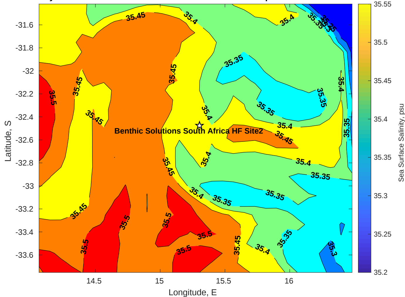
Surface Salinity for Benthic Solutions South Africa HF Site2 at 05-Apr-2025 00:00:00
