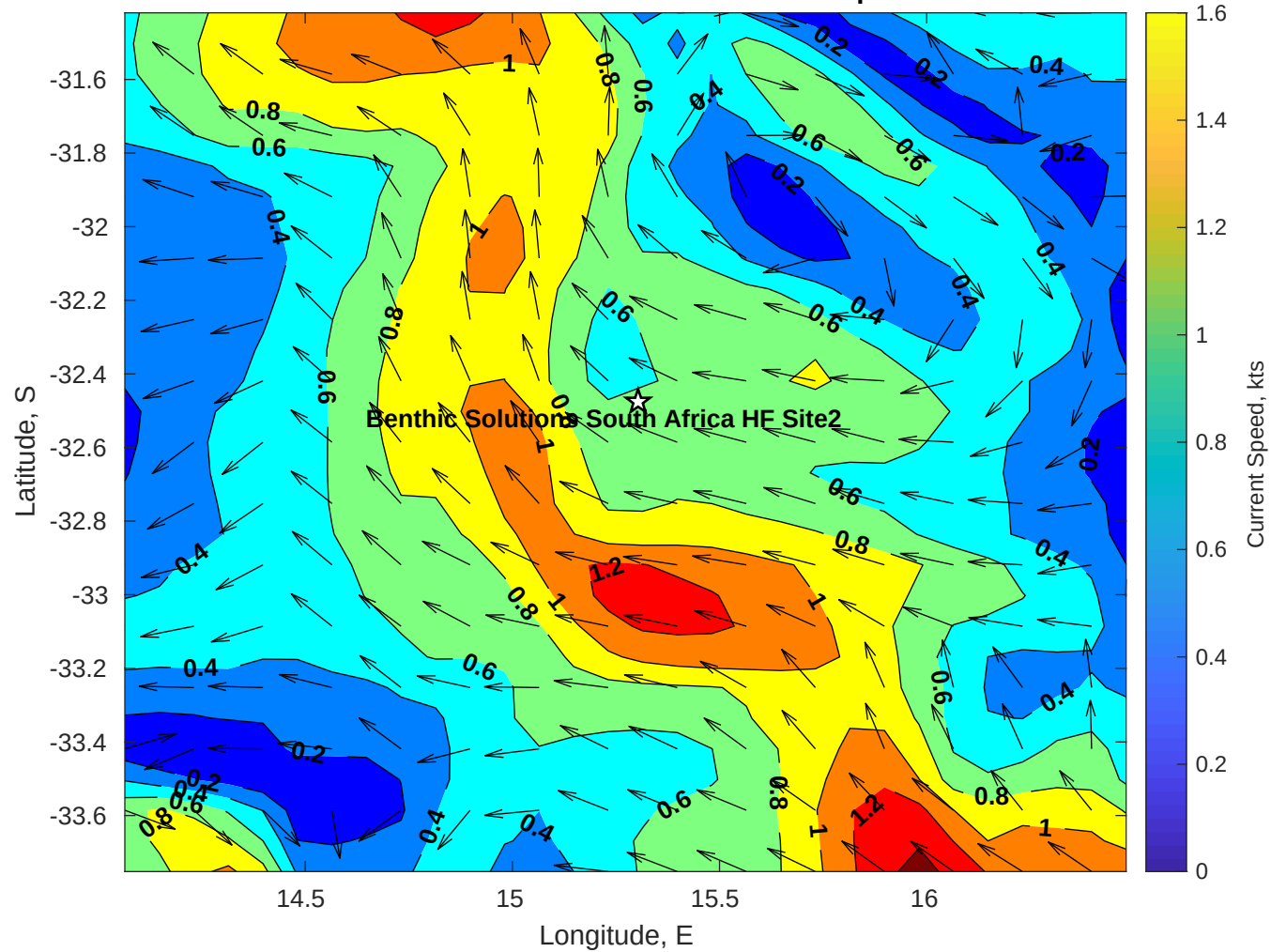
Surface Currents for Benthic Solutions South Africa HF Site2 at 05-Apr-2025 00:00:00
