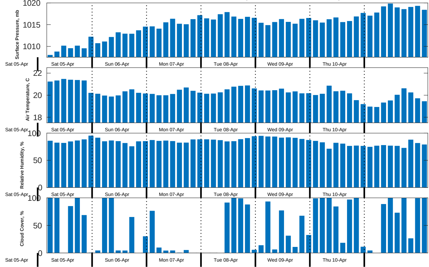
Met Forecast for Benthic Solutions South Africa HF Site2 from 06-Apr-2025 00:00:00 to 13-Apr-2025 00:00:00
