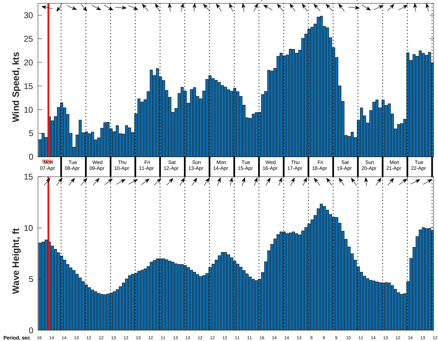
Wind & Wave Forecast for Benthic Solutions South Africa HF Site2 from 06-Apr-2025 02:00:00 to 22-Apr-2025 02:00:00
