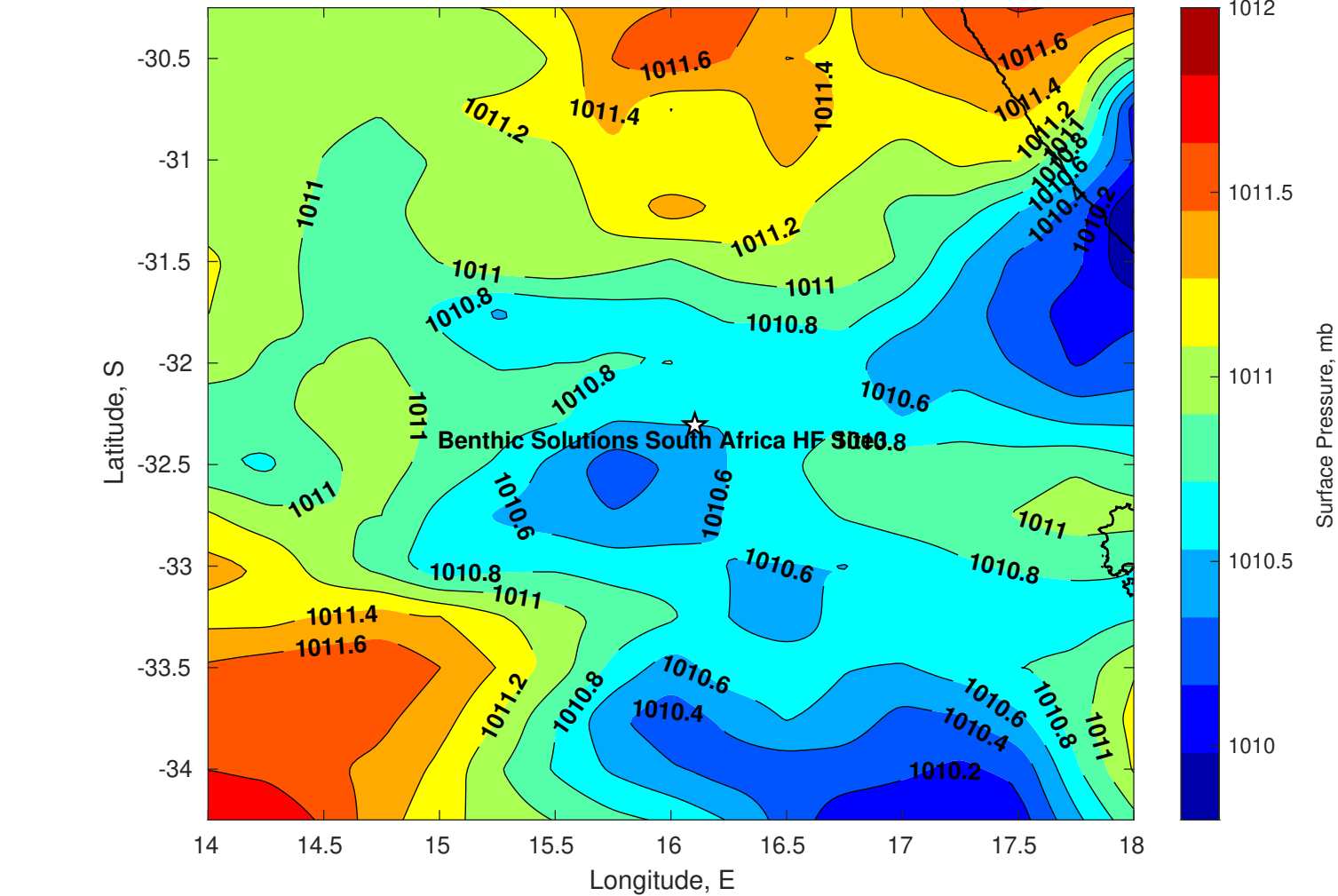
Surface Pressure (mb) for Benthic Solutions South Africa HF Site3 at 07-Apr-2025 00:00:00
