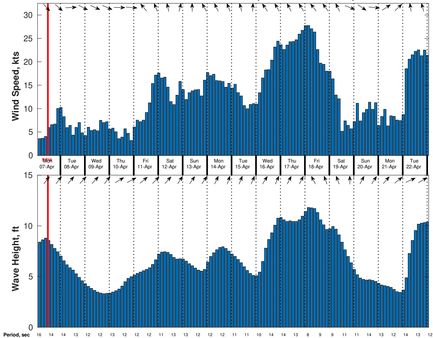
Wind & Wave Forecast for Benthic Solutions South Africa HF Site3 from 06-Apr-2025 02:00:00 to 22-Apr-2025 02:00:00
