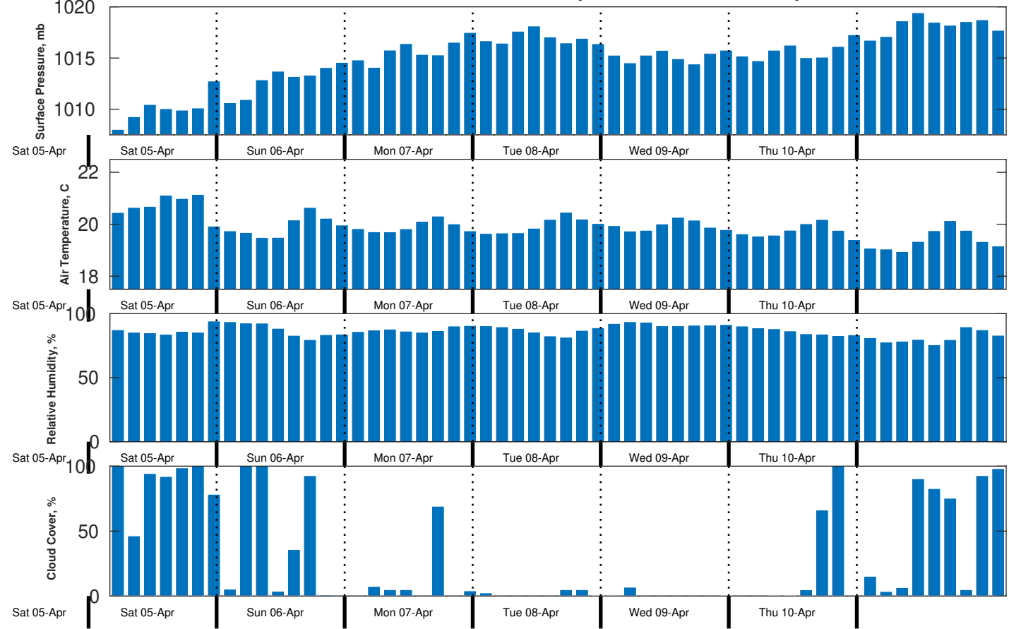
Met Forecast for Benthic Solutions South Africa HF Site3 from 06-Apr-2025 00:00:00 to 13-Apr-2025 00:00:00
