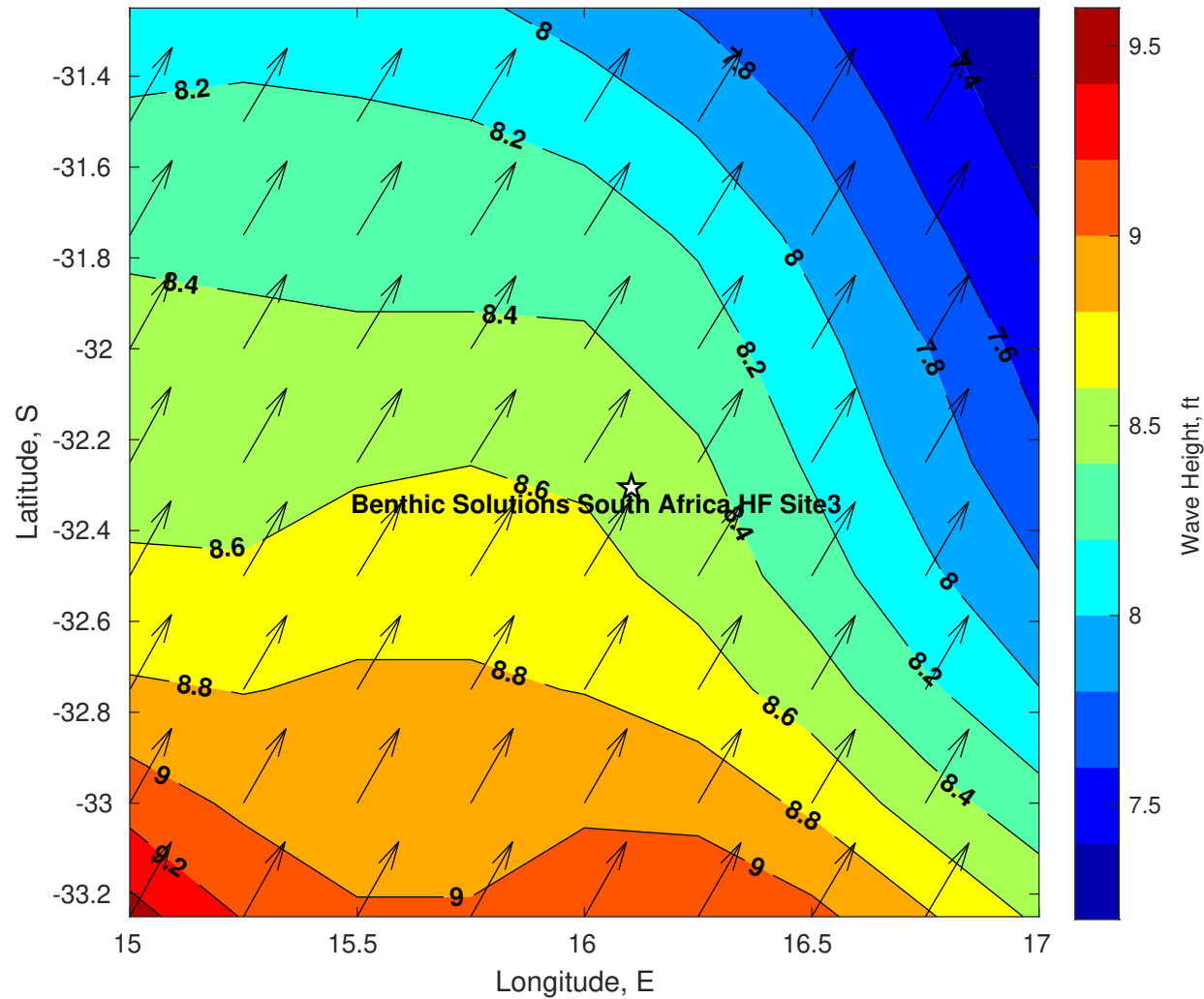
Wave Height (ft) for Benthic Solutions South Africa HF Site3 at 06-Apr-2025 09:00:00
