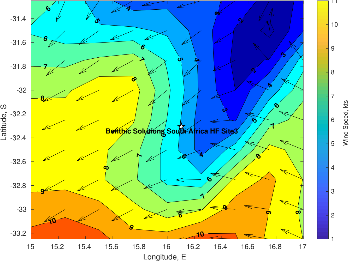
Winds (kts) for Benthic Solutions South Africa HF Site3 at 06-Apr-2025 09:00:00
