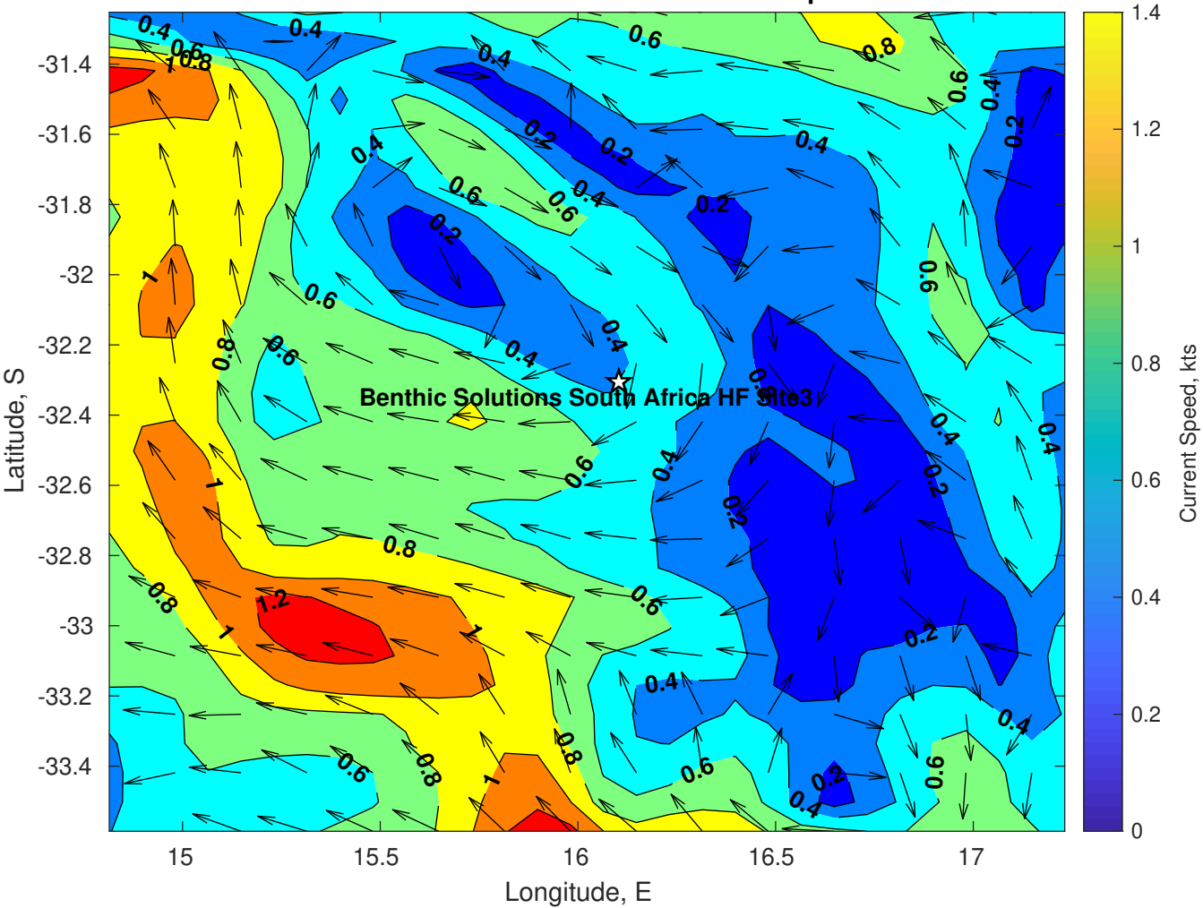
Surface Currents for Benthic Solutions South Africa HF Site3 at 05-Apr-2025 00:00:00
