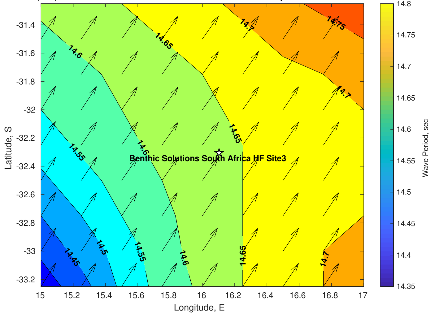
Wave Period (sec) for Benthic Solutions South Africa HF Site3 at 06-Apr-2025 09:00:00
