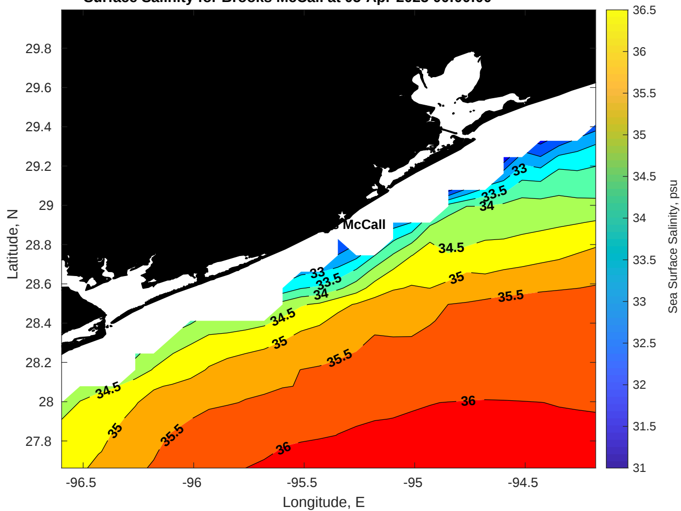
Surface Salinity for Brooks McCall at 05-Apr-2025 00:00:00
