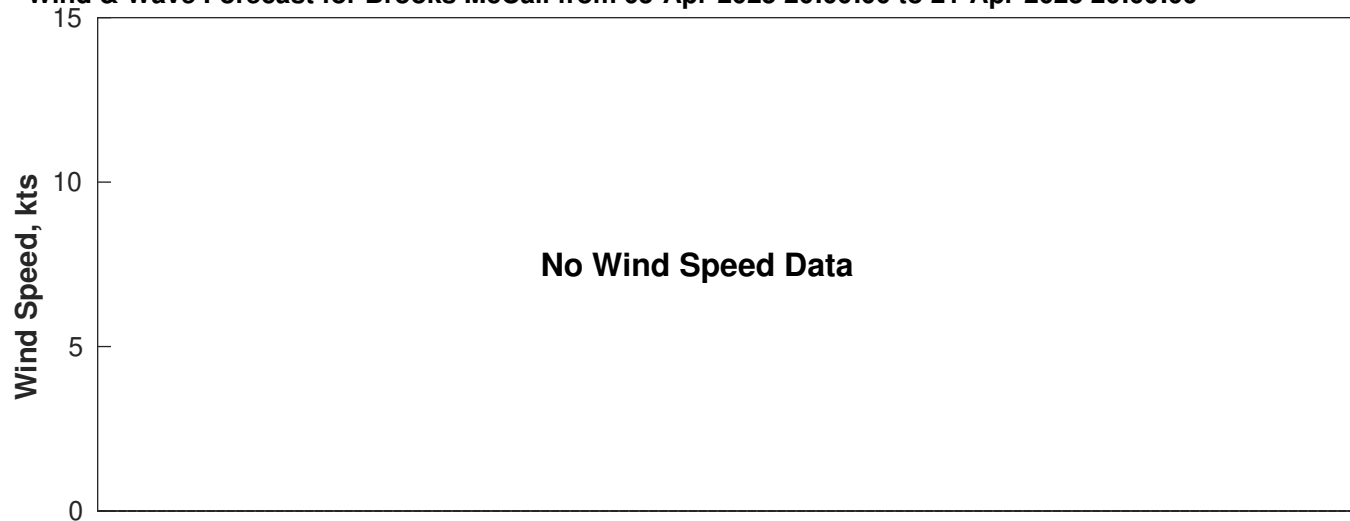
Wind & Wave Forecast for Brooks McCall from 05-Apr-2025 20:00:00 to 21-Apr-2025 20:00:00
