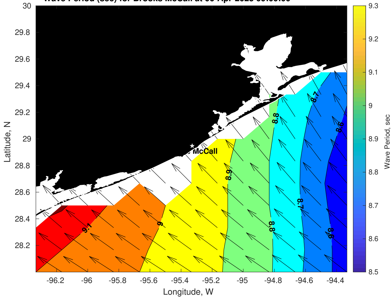
Wave Period (sec) for Brooks McCall at 06-Apr-2025 09:00:00
