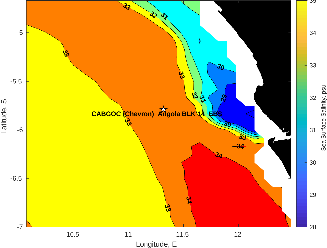
Surface Salinity for CABGOC (Chevron) Angola BLK 14 EBS at 05-Apr-2025 00:00:00
