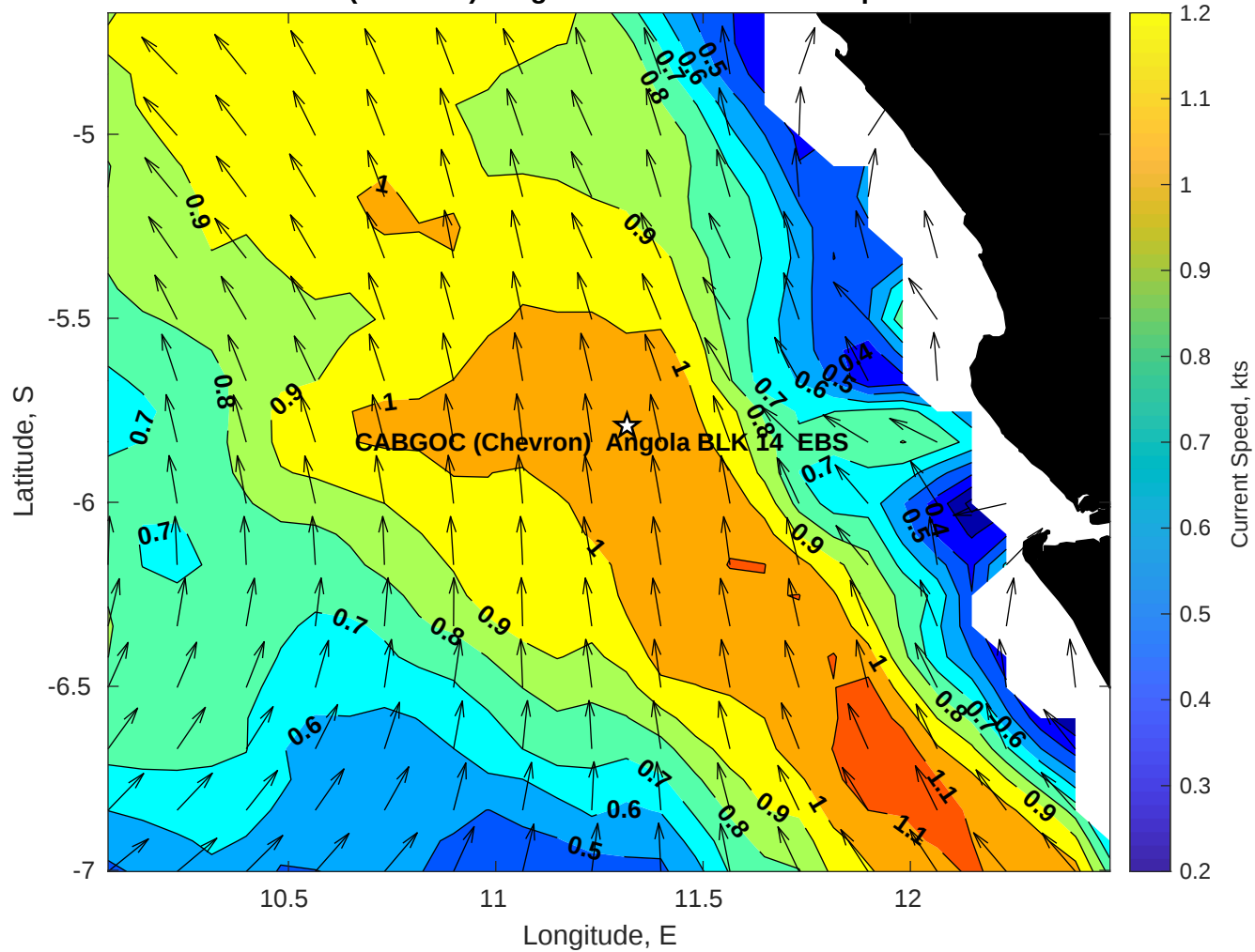
Surface Currents for CABGOC (Chevron) Angola BLK 14 EBS at 05-Apr-2025 00:00:00
